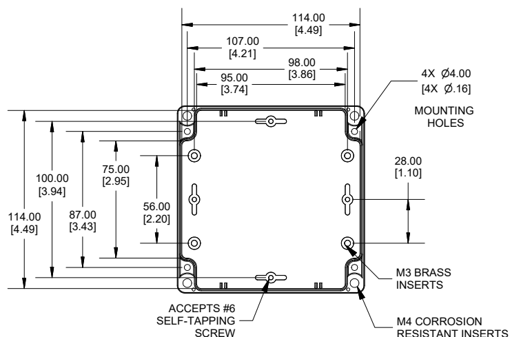
INSIDE BOX
