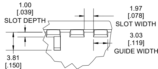
DETAIL D
