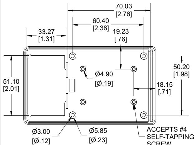
INSIDE BOTTOM
