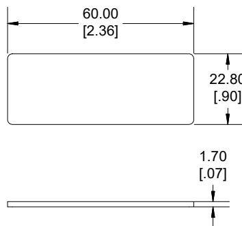
END PANEL
