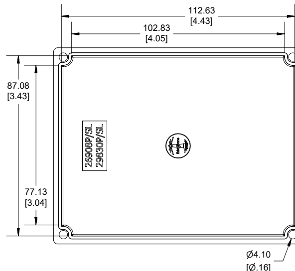
INSIDE LID VIEW
