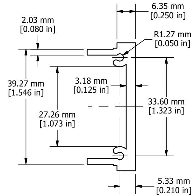
PROFILE VIEW
