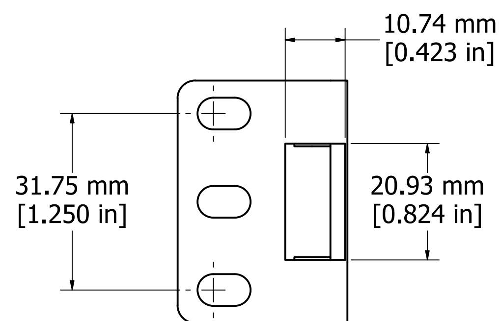
(1) REAR SUPPORT BRACKET FRONT VIEW
