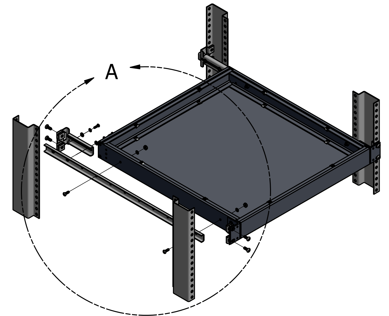
ISOMETRIC VIEW (EXPLODED)
