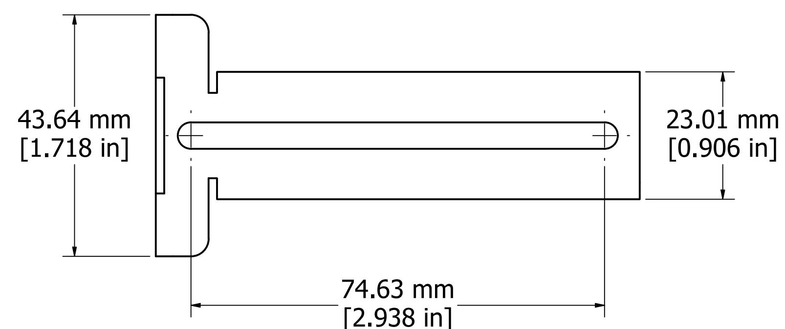
SIDE VIEW
