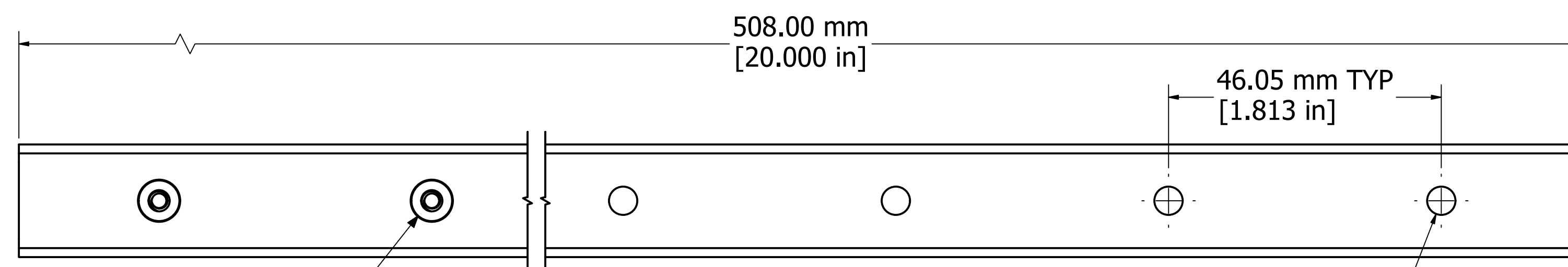
(2) REAR EXTENSION BRACKET SIDE VIEW
