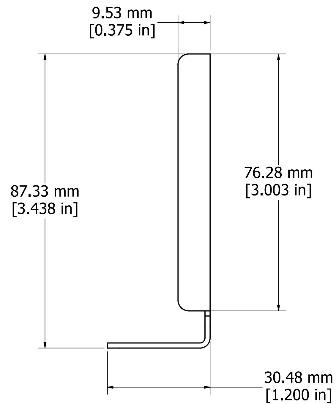
TOP VIEW
