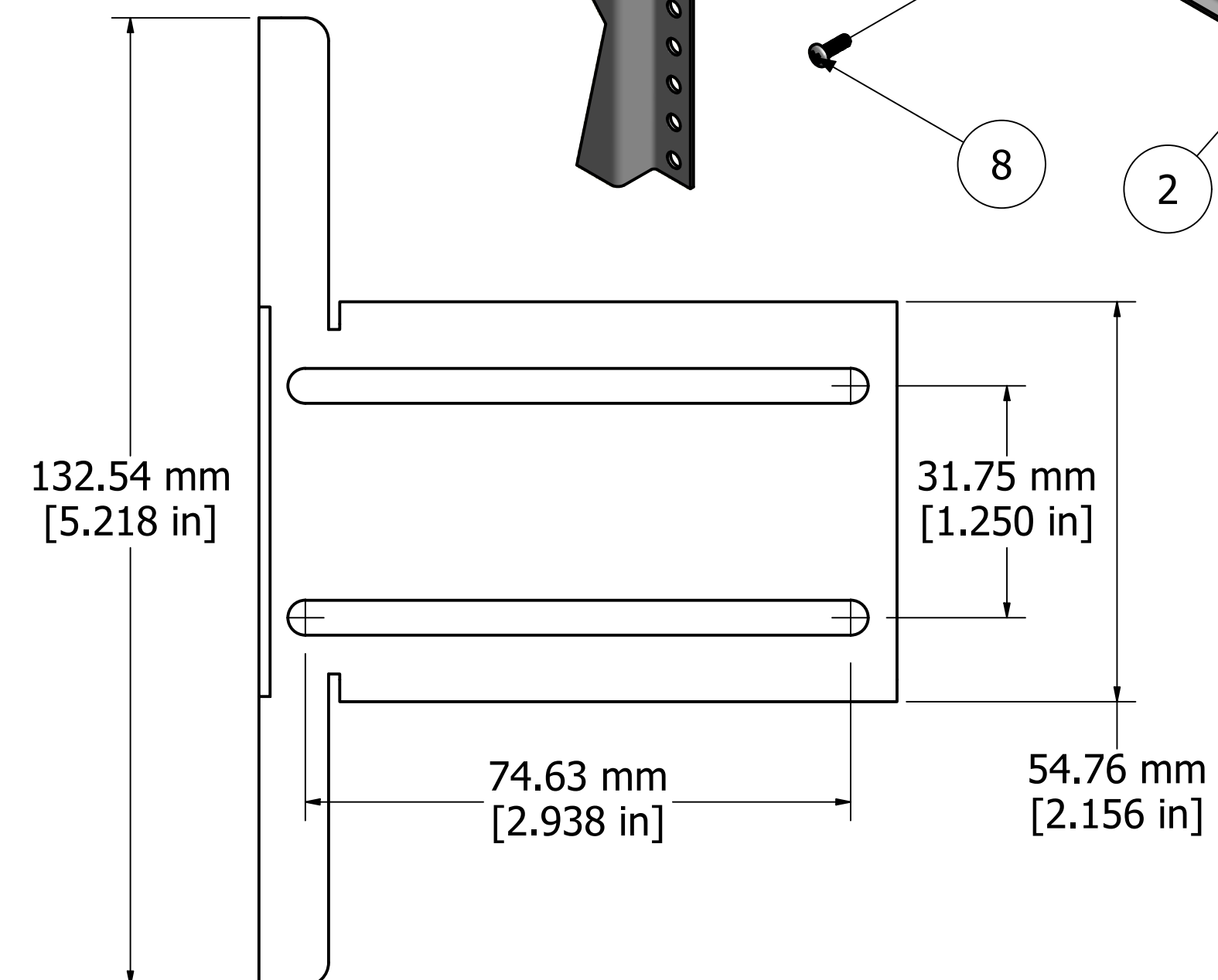
SIDE VIEW
