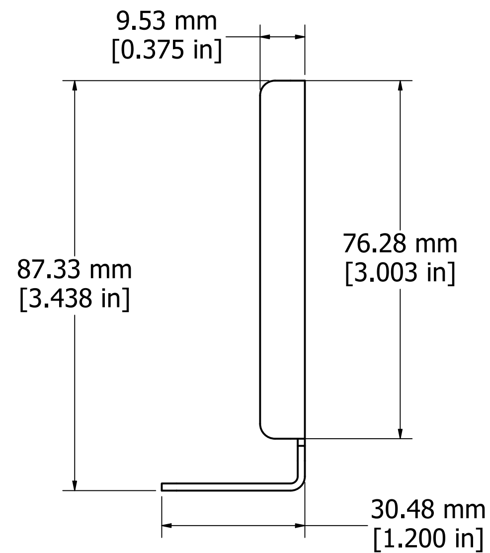
TOP VIEW
