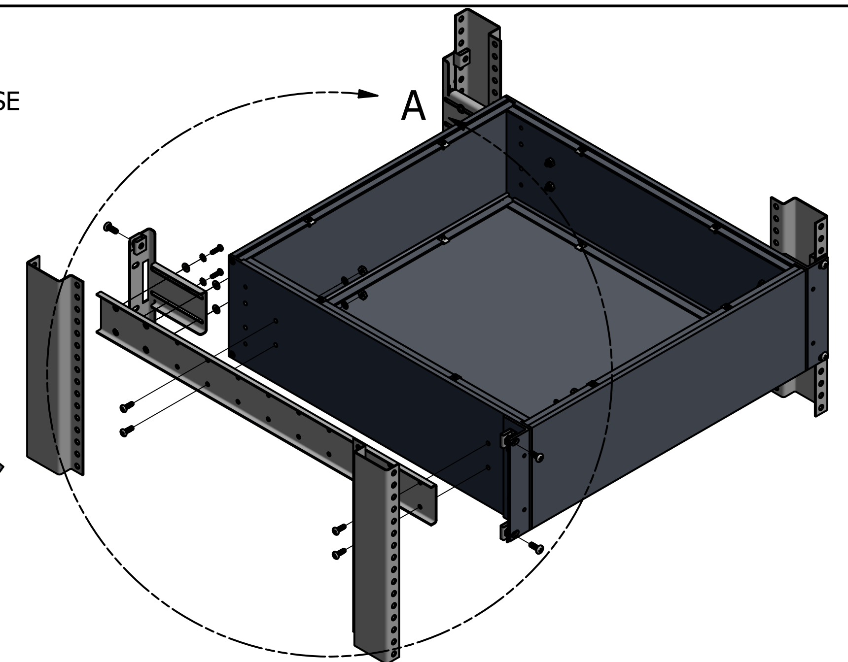
ISOMETRIC VIEW (EXPLODED)
