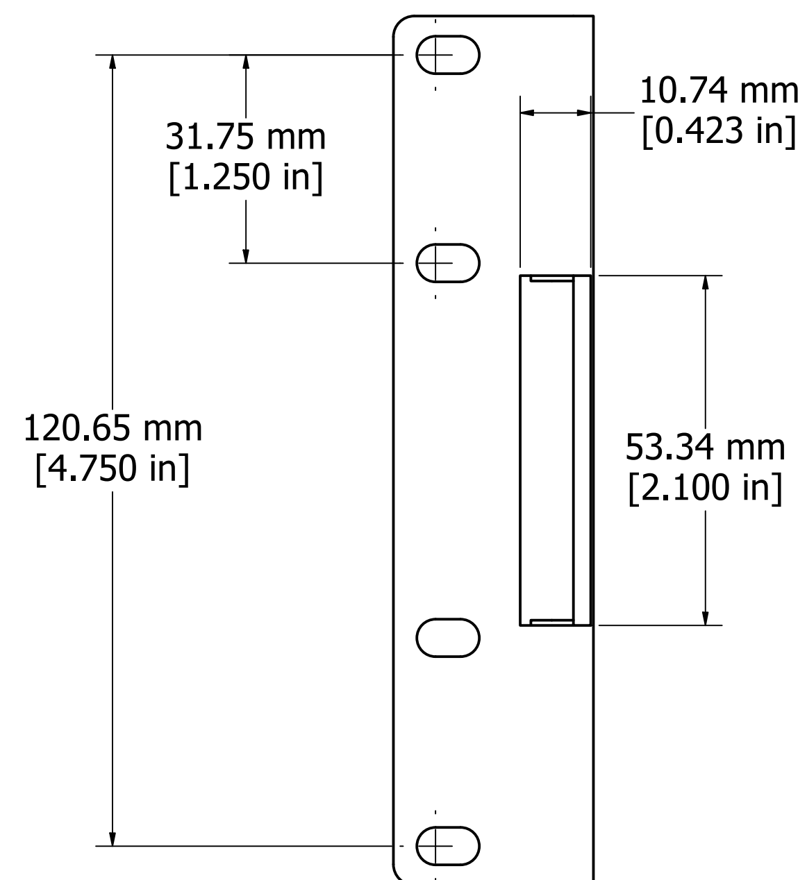
(1) REAR SUPPORT BRACKET FRONT VIEW
