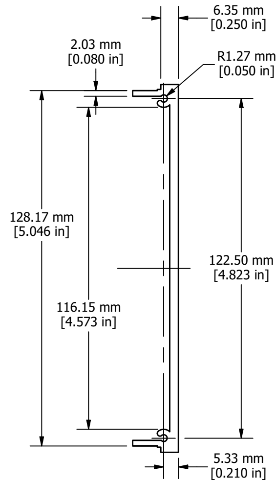
PROFILE VIEW
