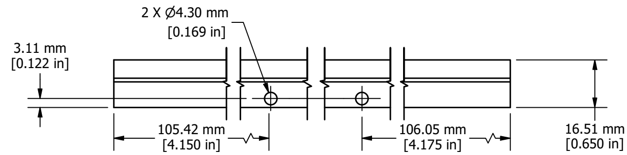
TOP VIEW
