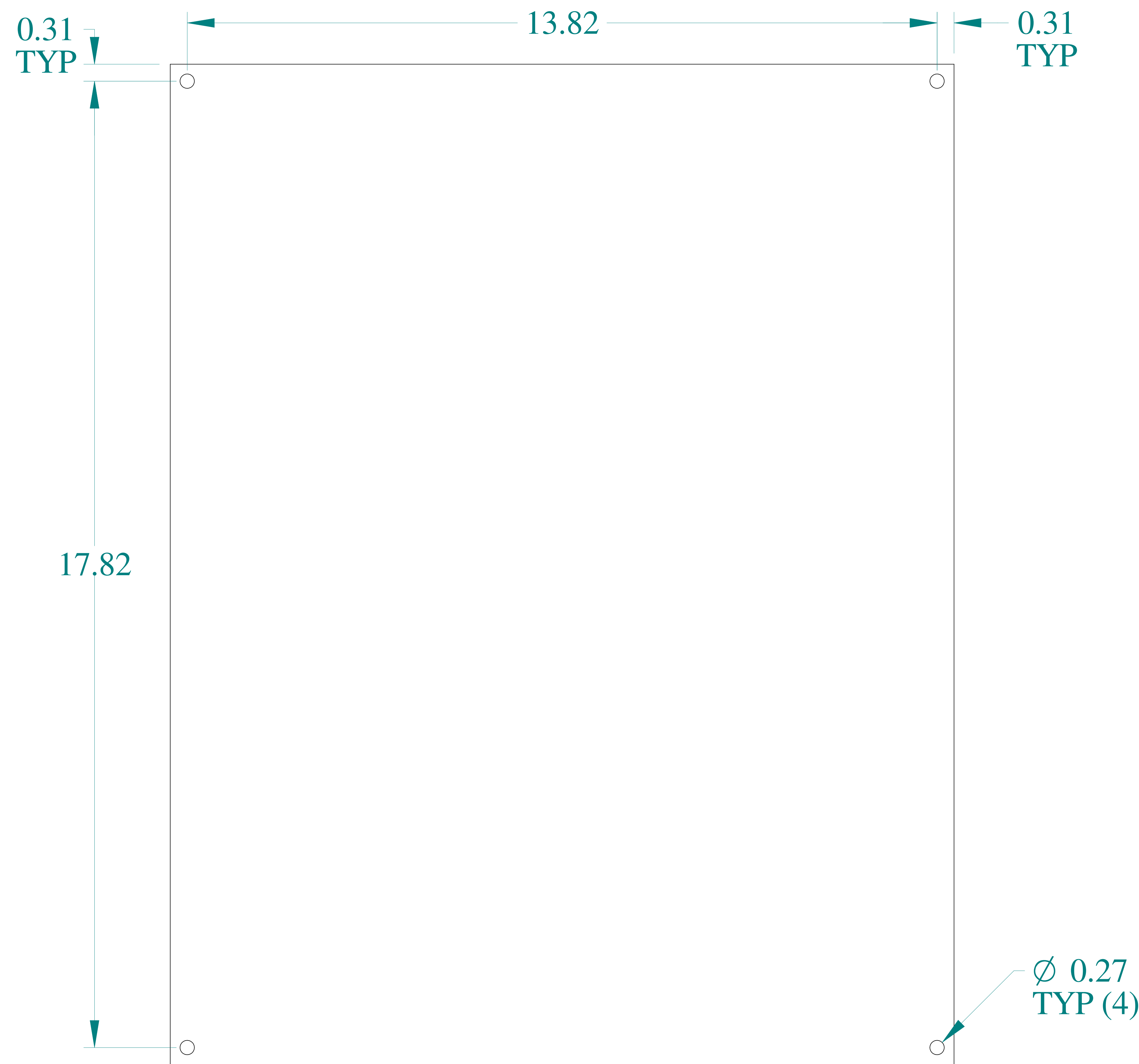
FRONT VIEW
