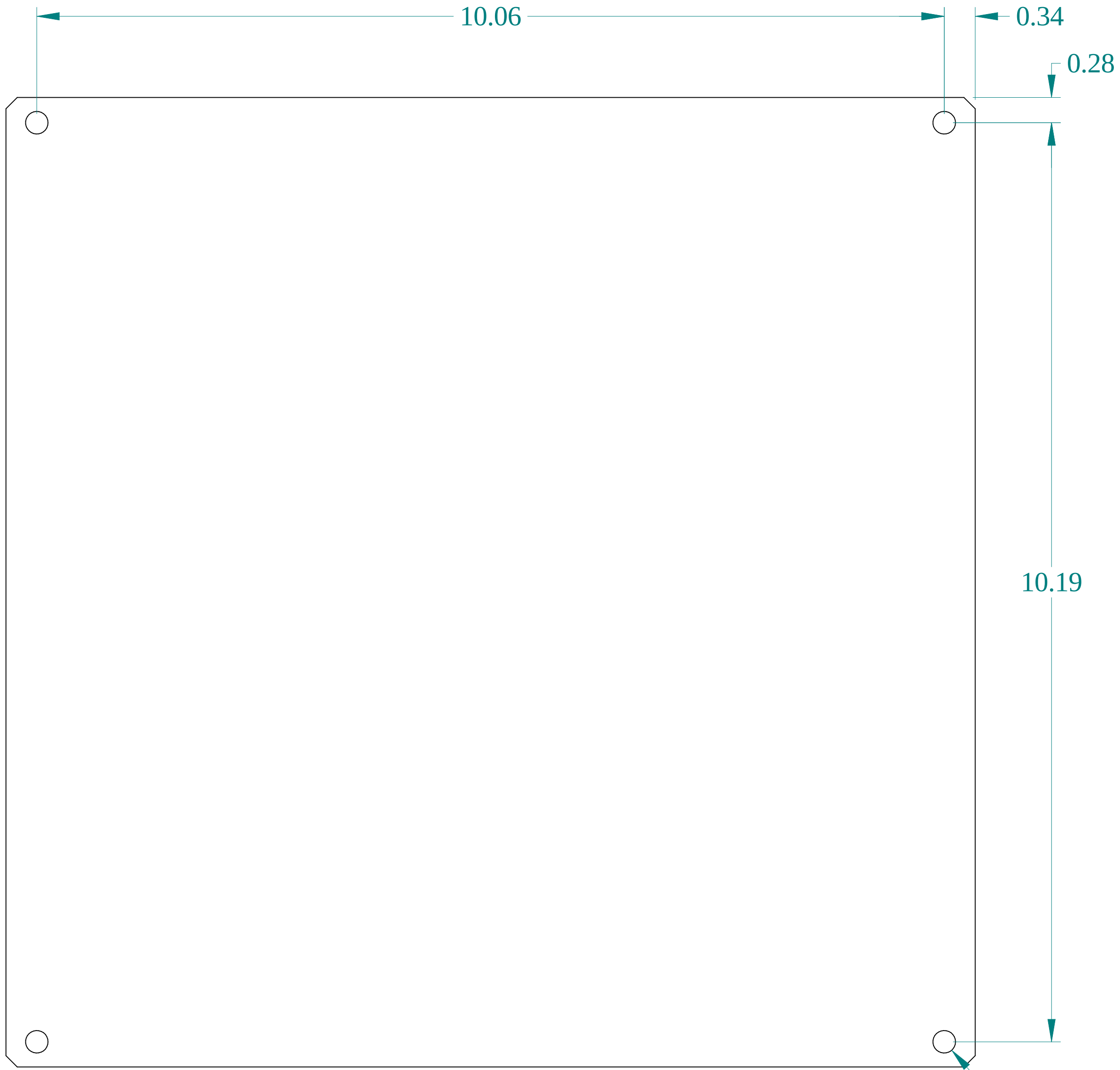
FRONT VIEW
