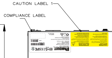
DETAIL A SCALE 1: 2
