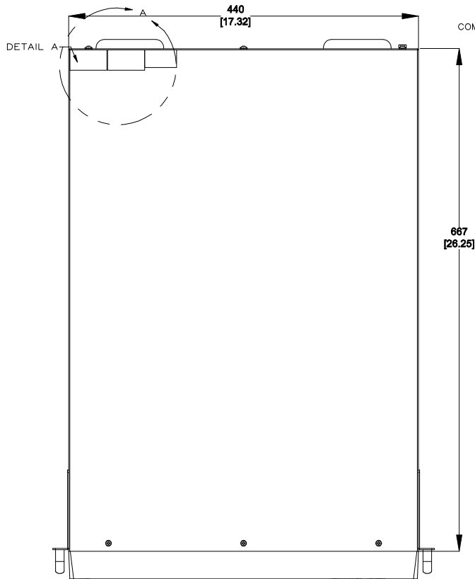
VIEW ROTATED 180°
