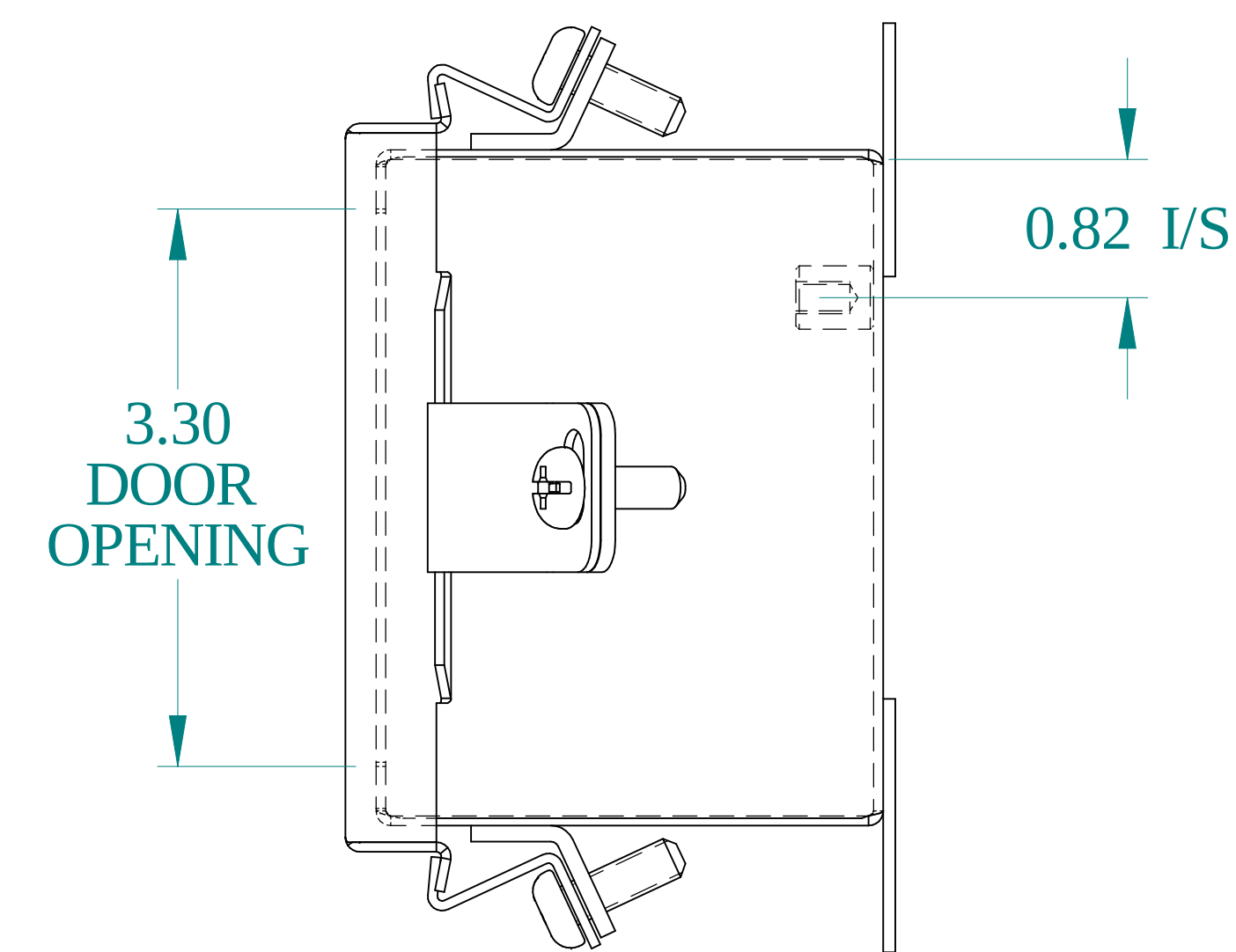
SIDE VIEW
