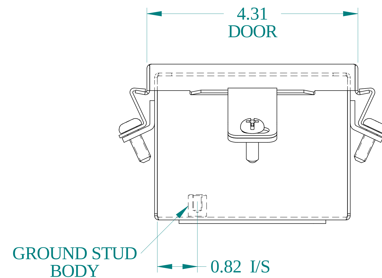
BOTTOM VIEW
