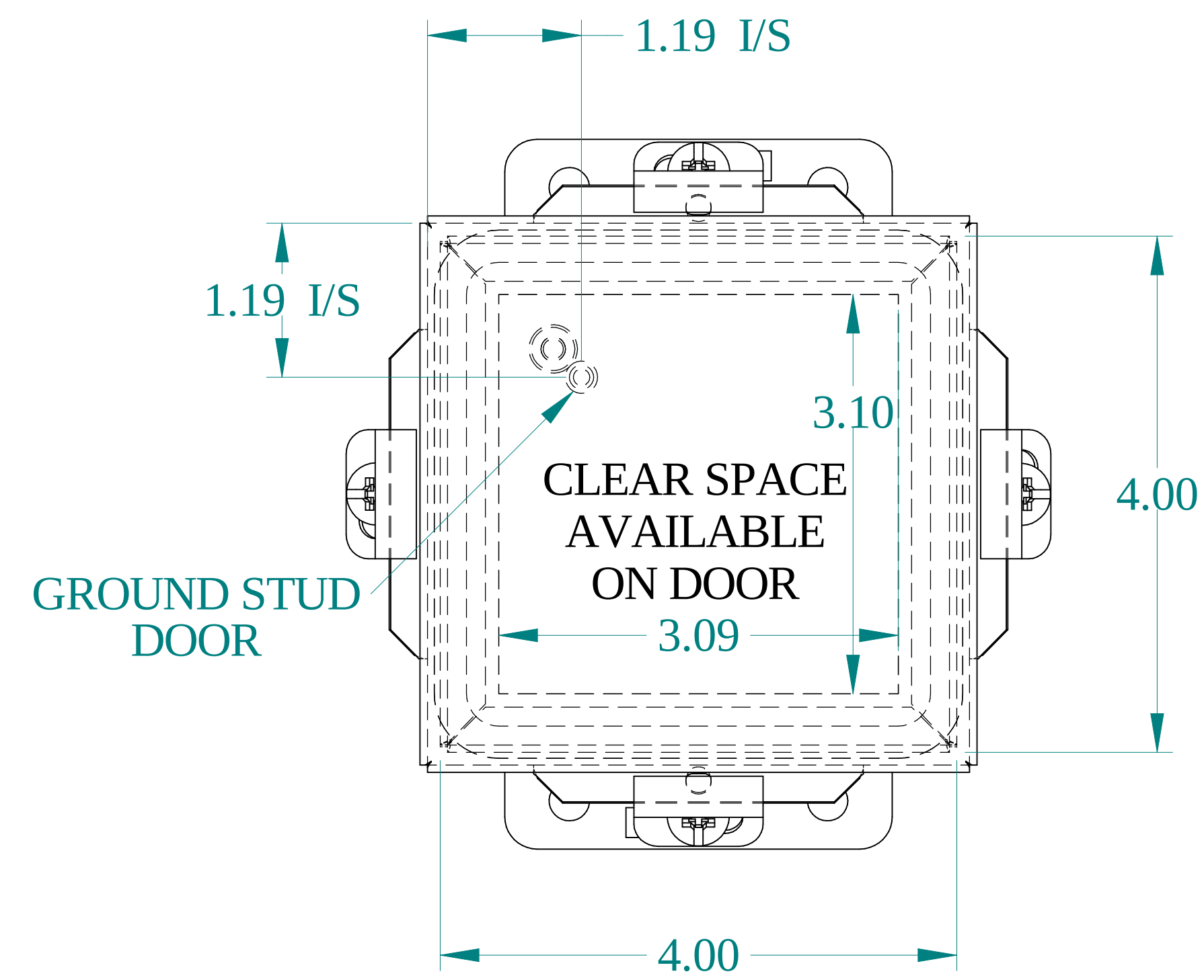
FRONT VIEW
