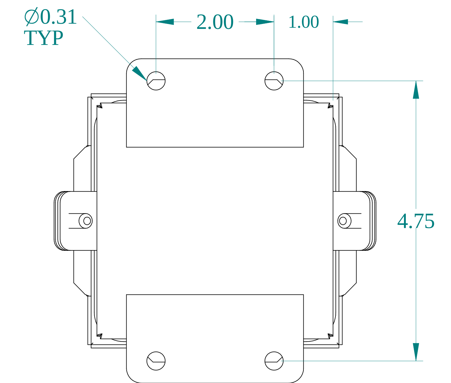
BACK VIEW
