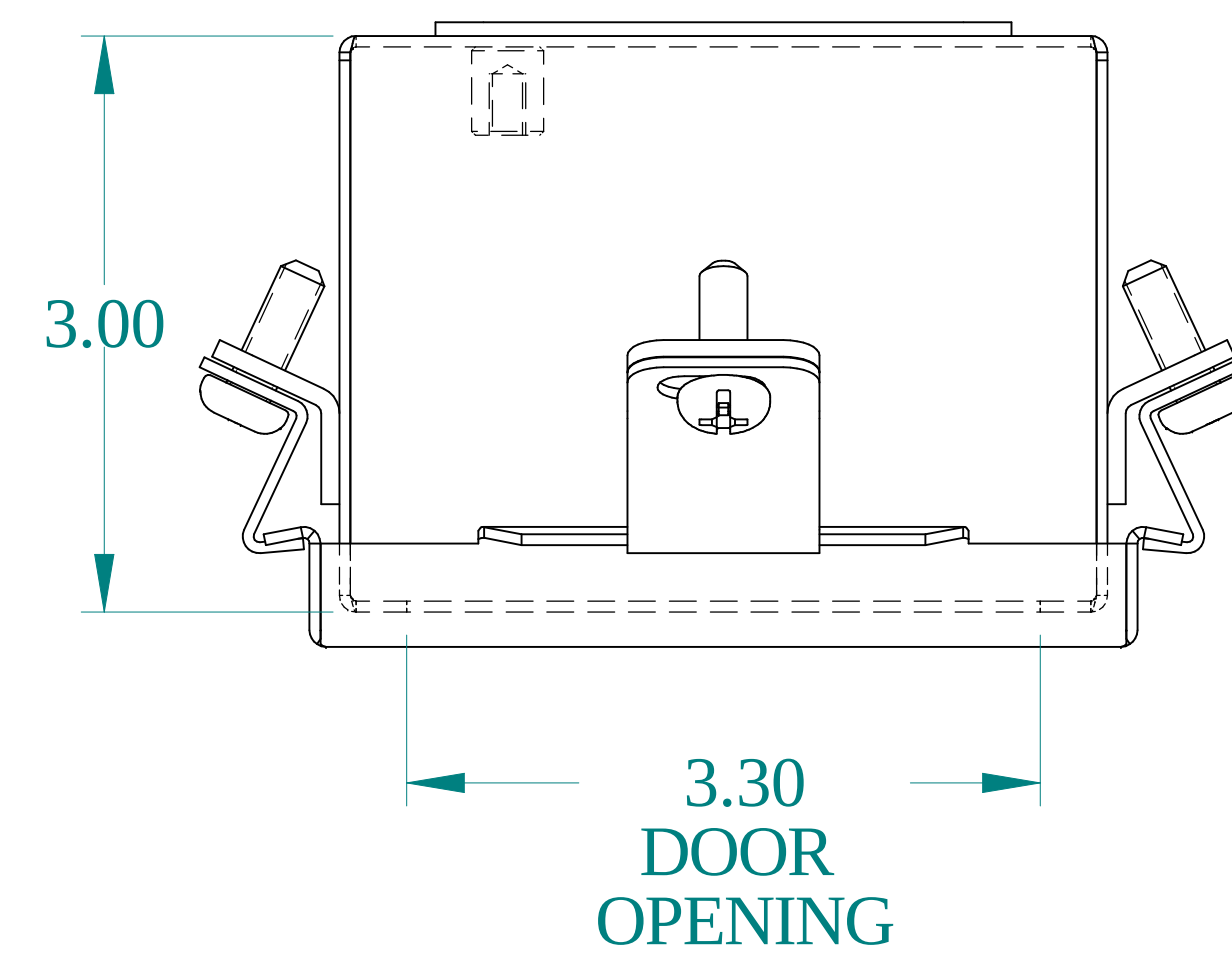
TOP VIEW
