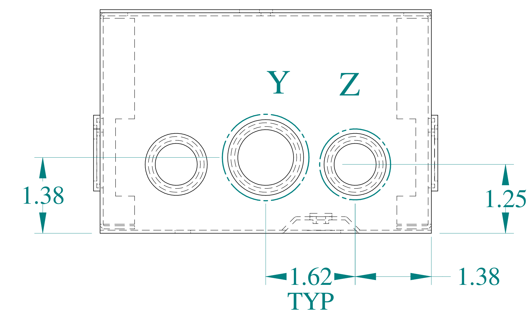
SIDE VIEW
