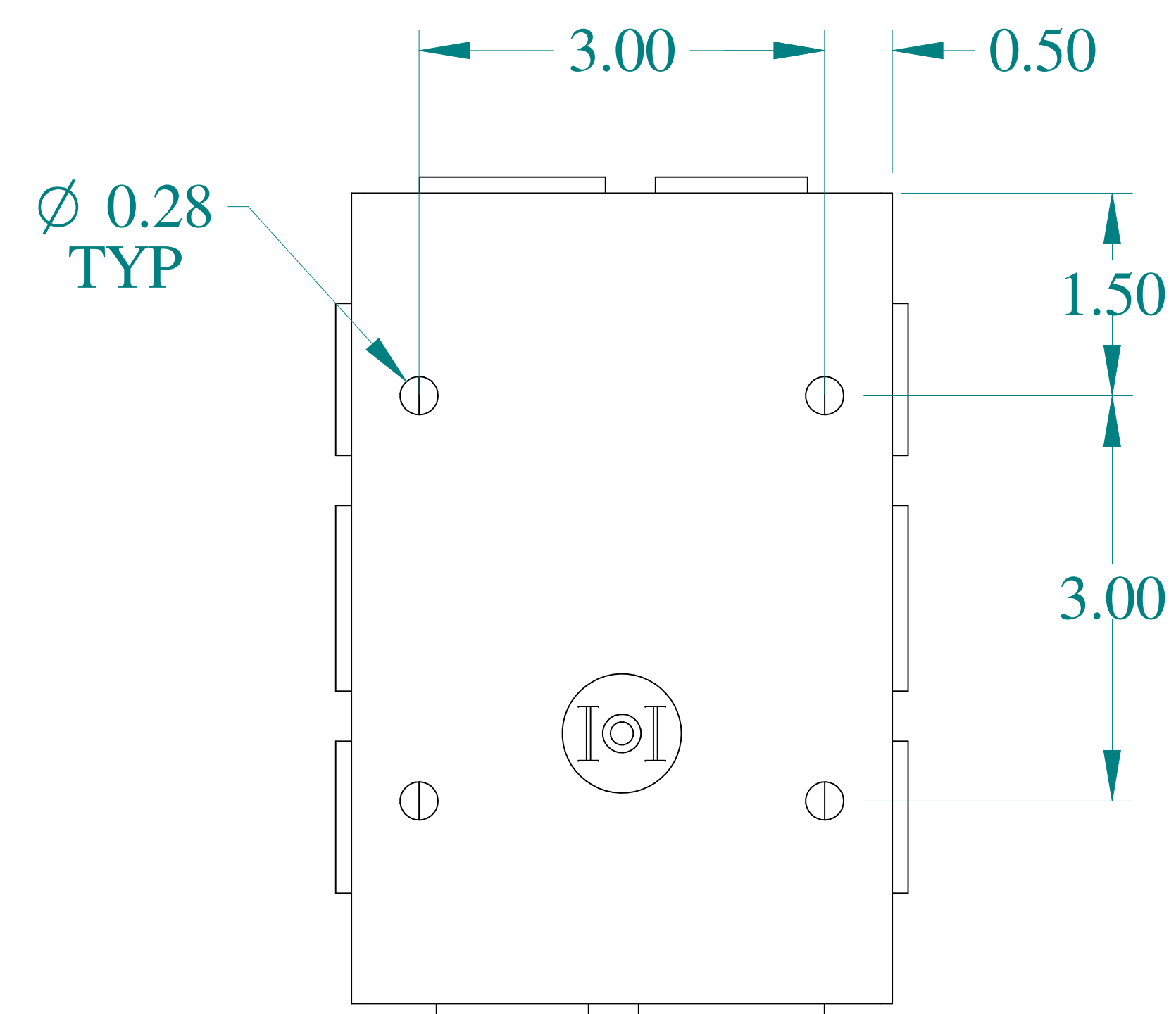
BOTTOM VIEW
