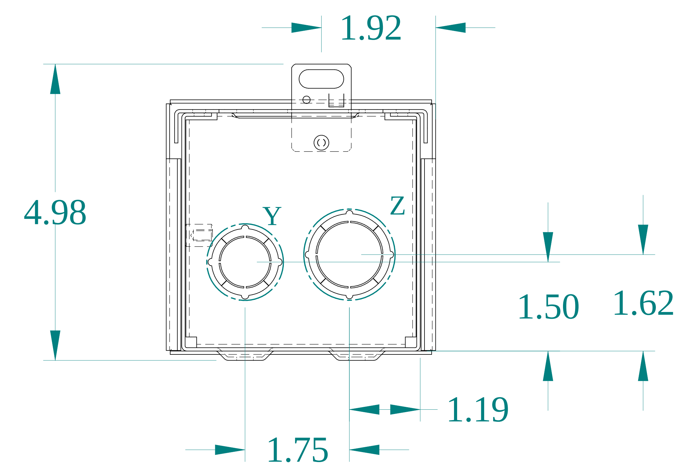
BOTTOM VIEW
