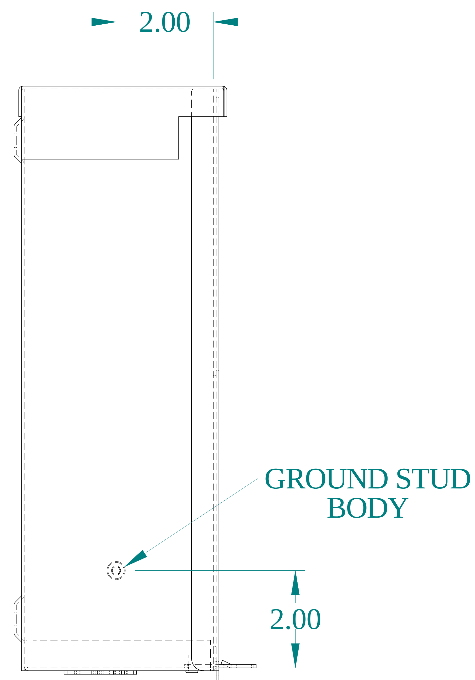
SIDE VIEW
