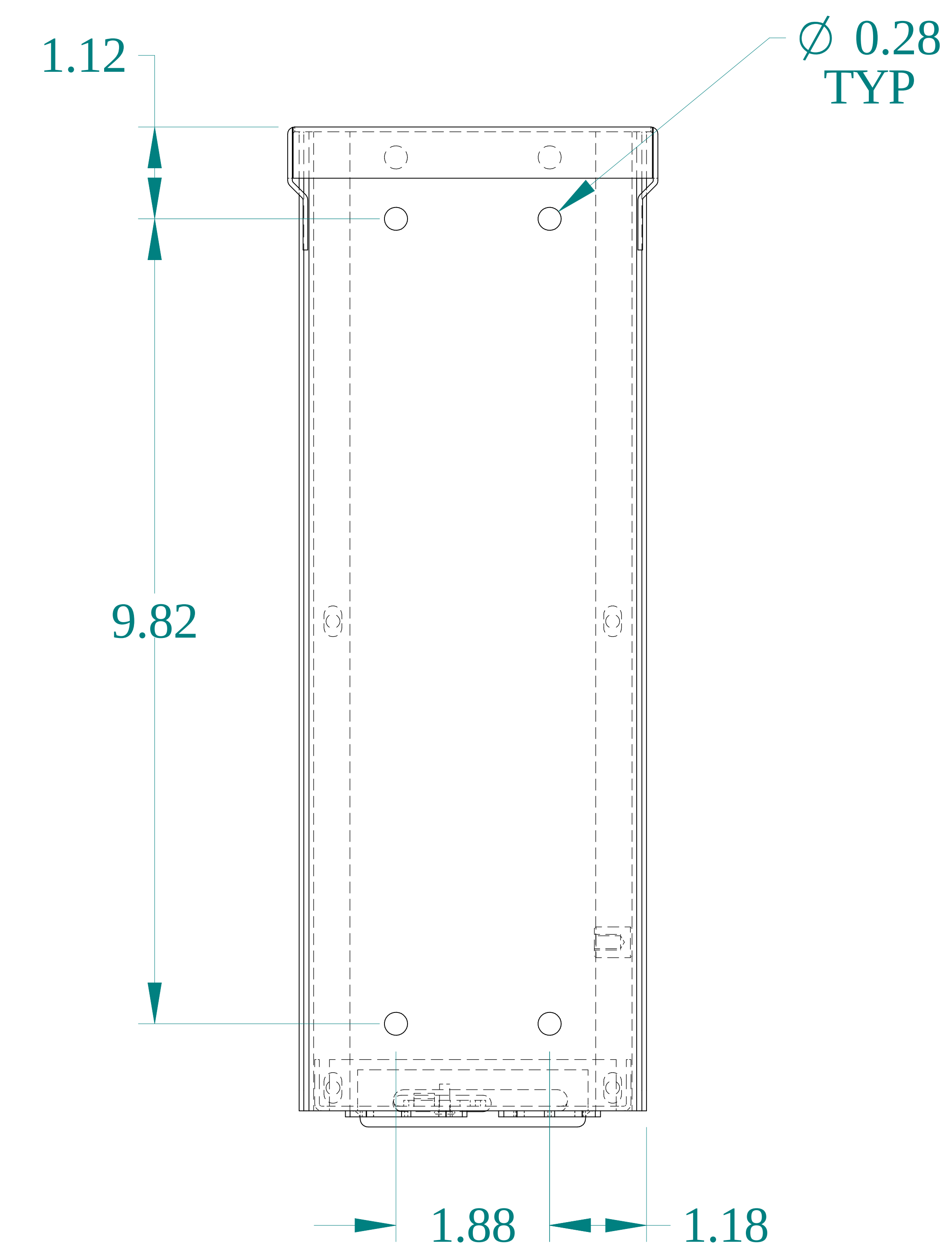
BACK VIEW
