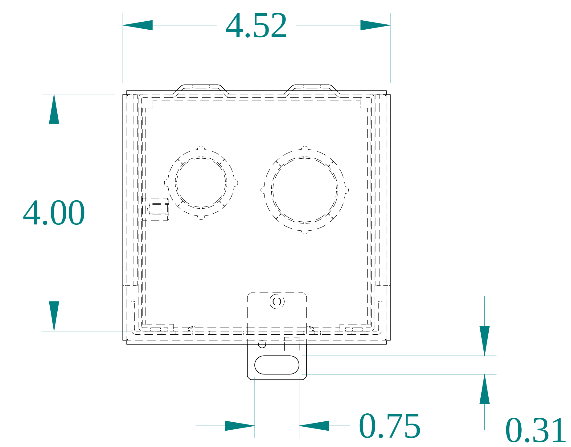
TOP VIEW
