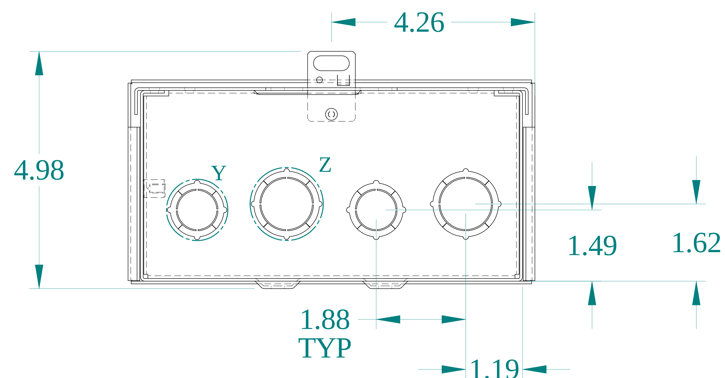
BOTTOM VIEW
