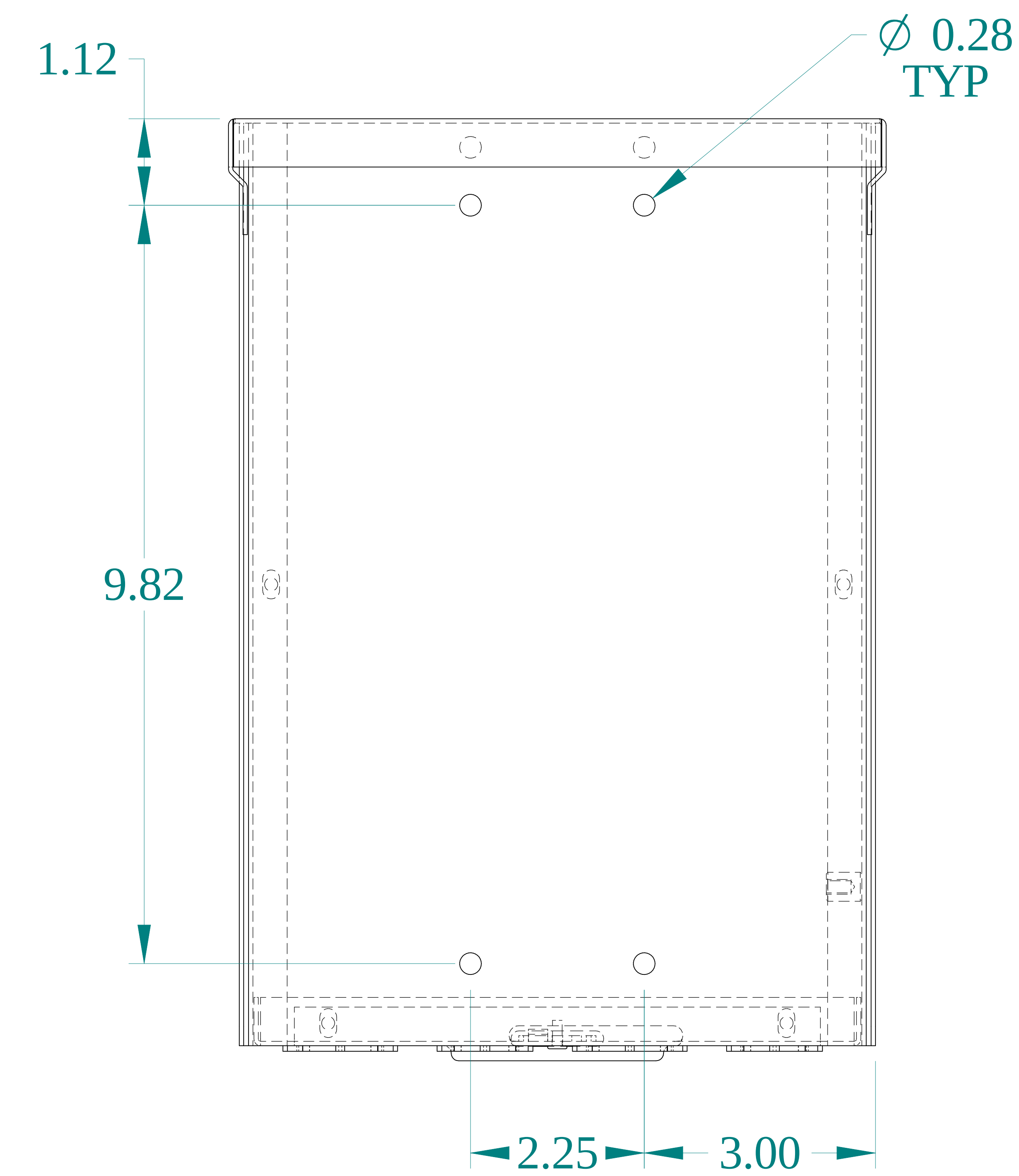
BACK VIEW
