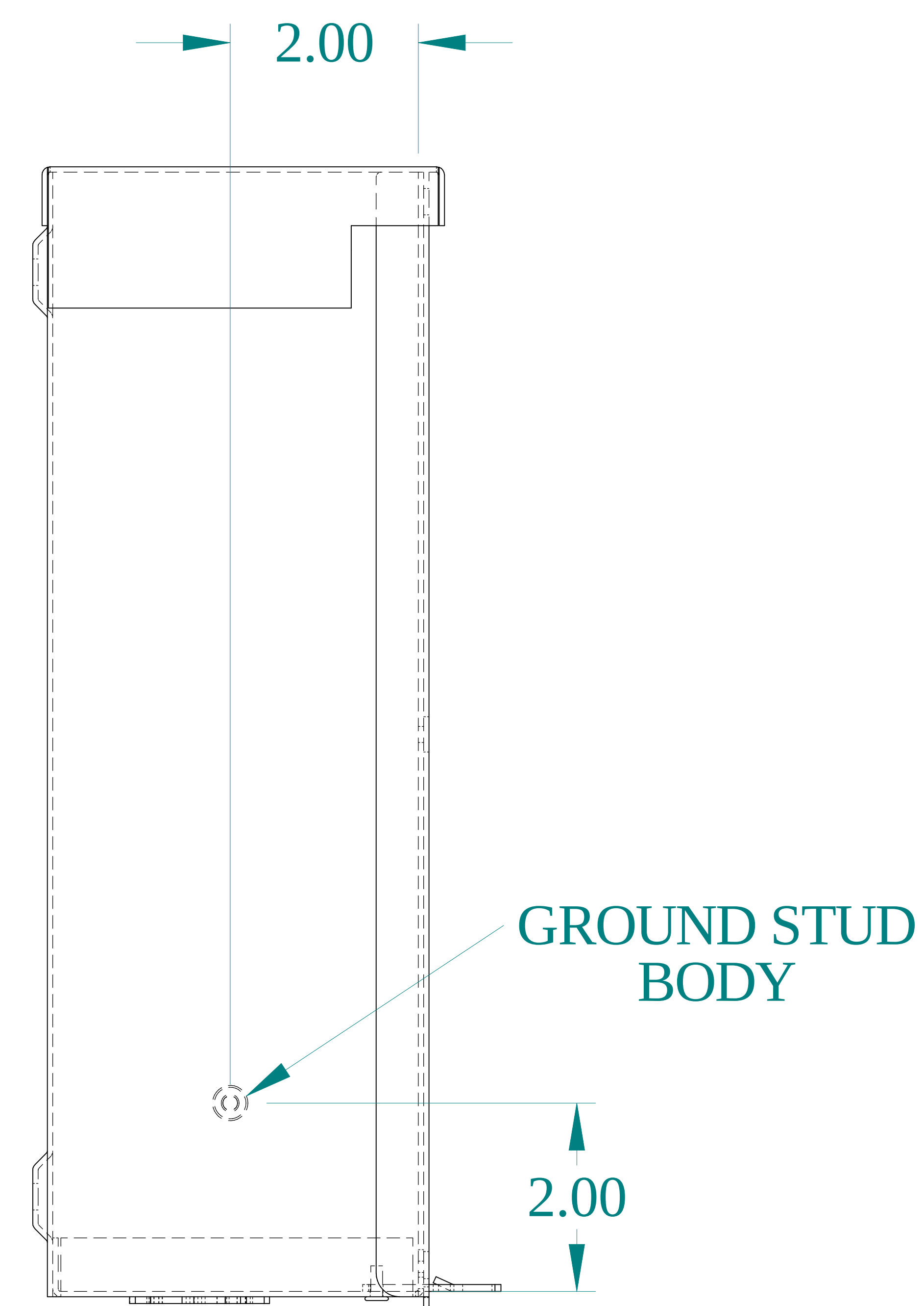
SIDE VIEW
