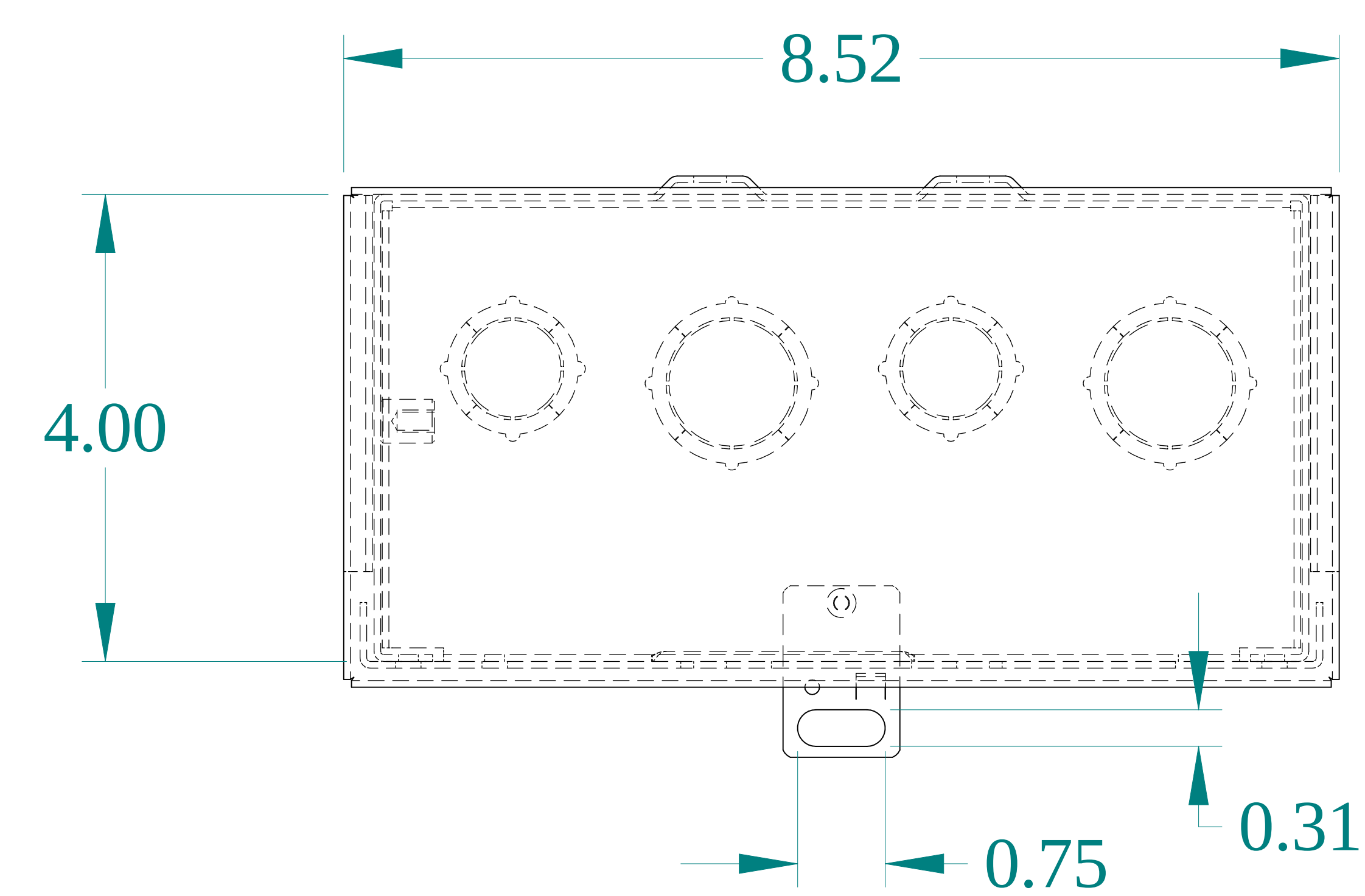
TOP VIEW
