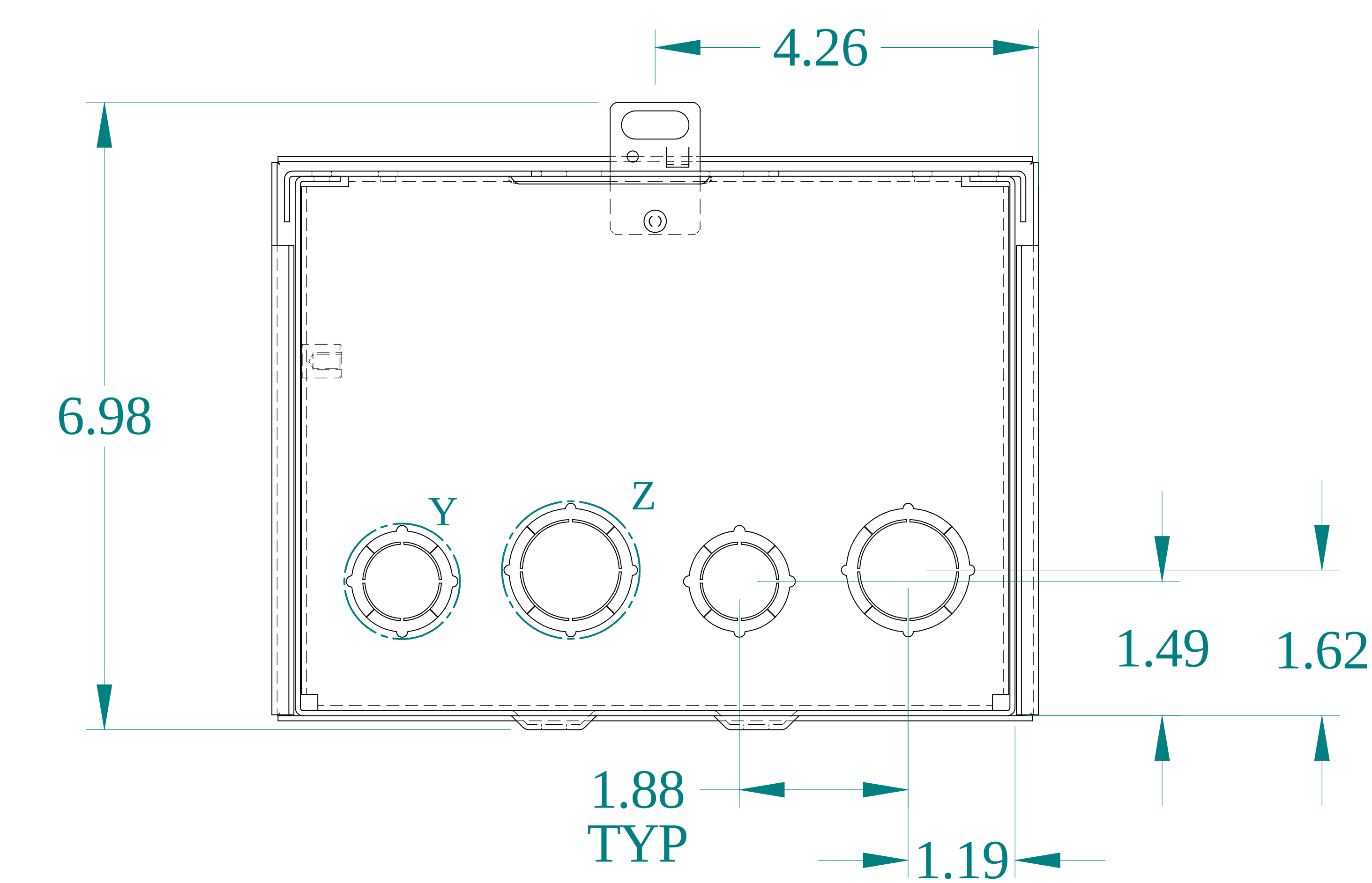
BOTTOM VIEW
