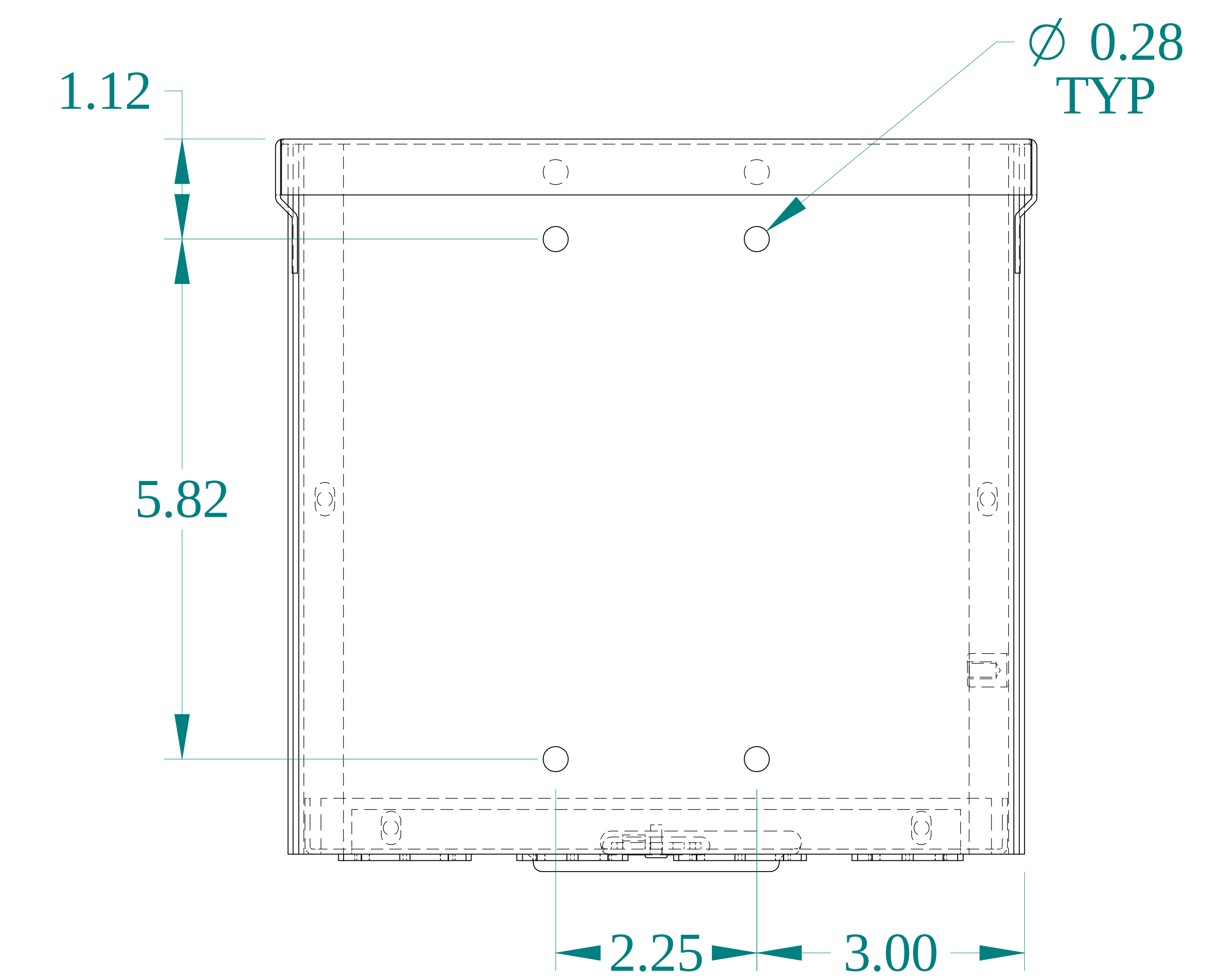
BACK VIEW
