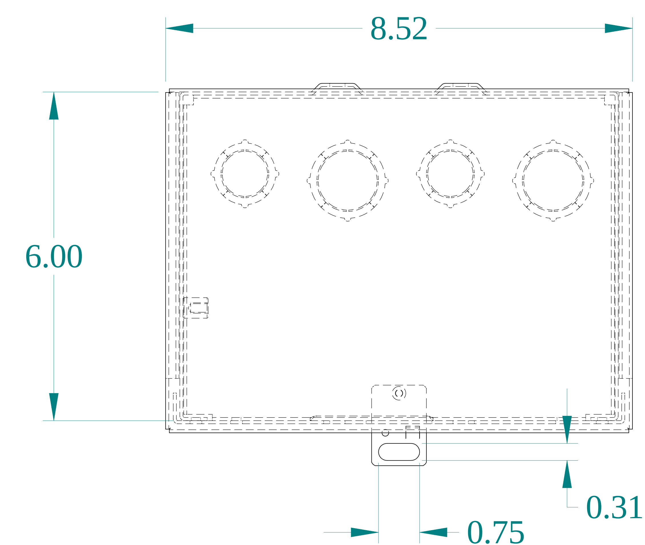
TOP VIEW
