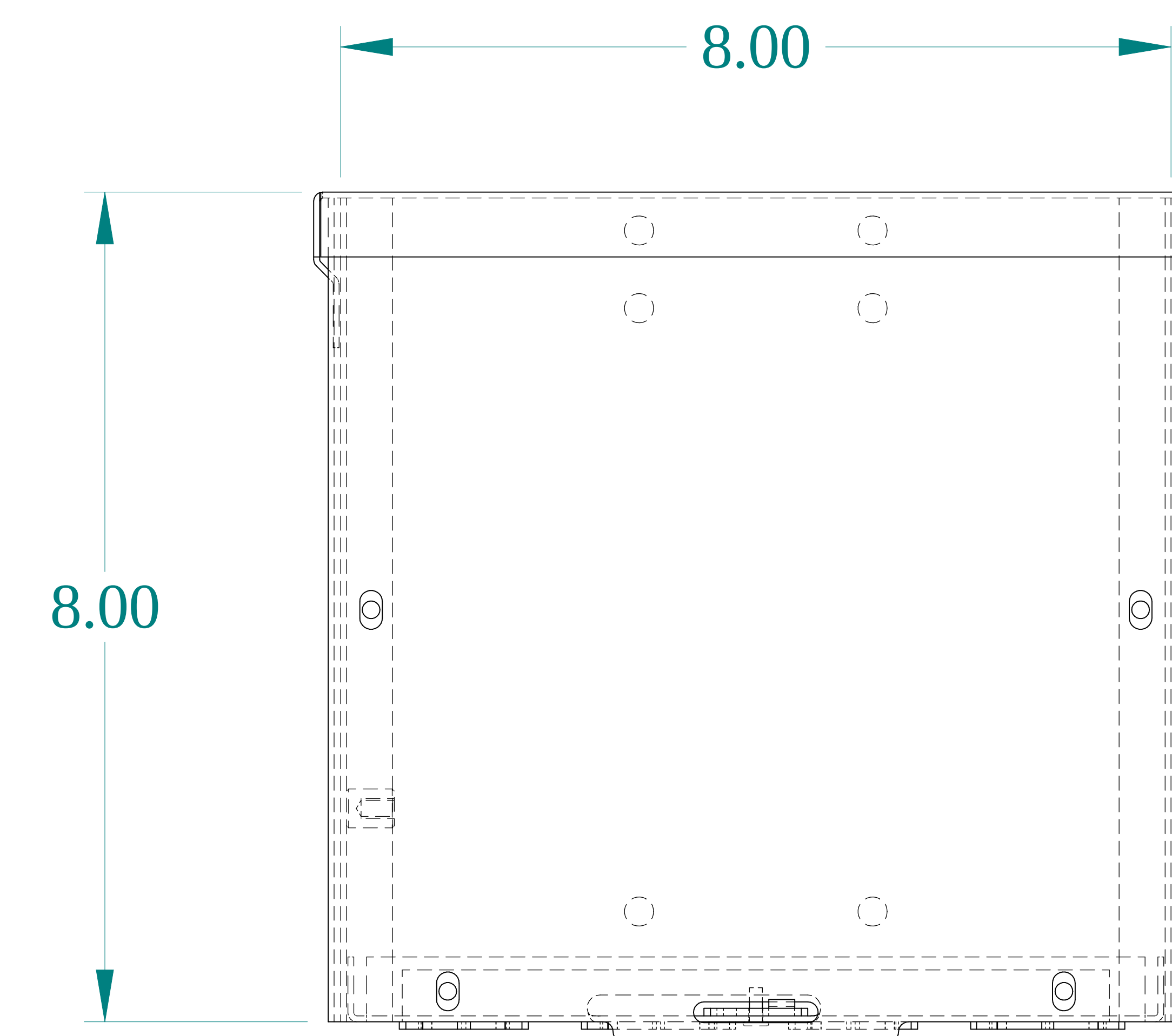
FRONT VIEW
