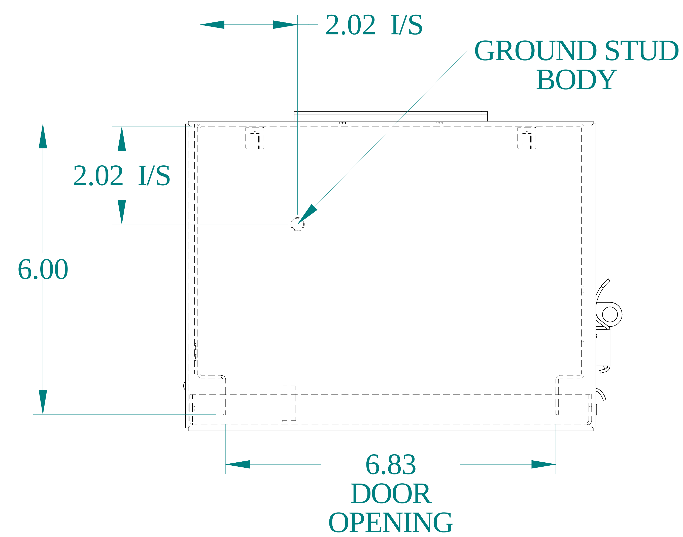
TOP VIEW
