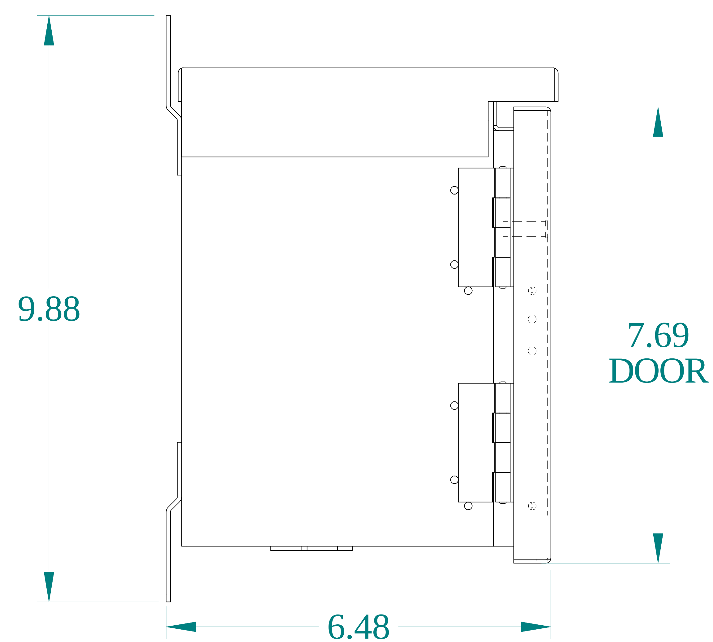
SIDE VIEW
