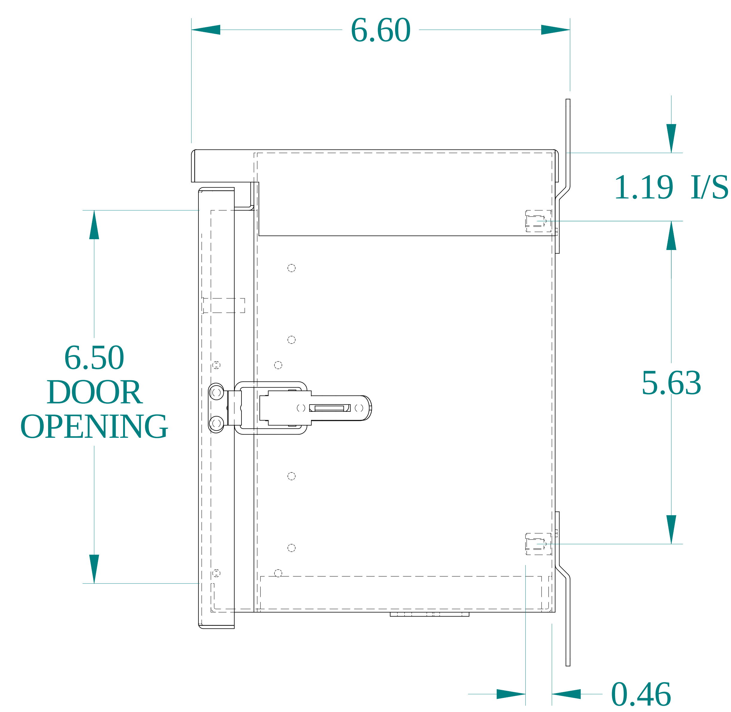
SIDE VIEW
