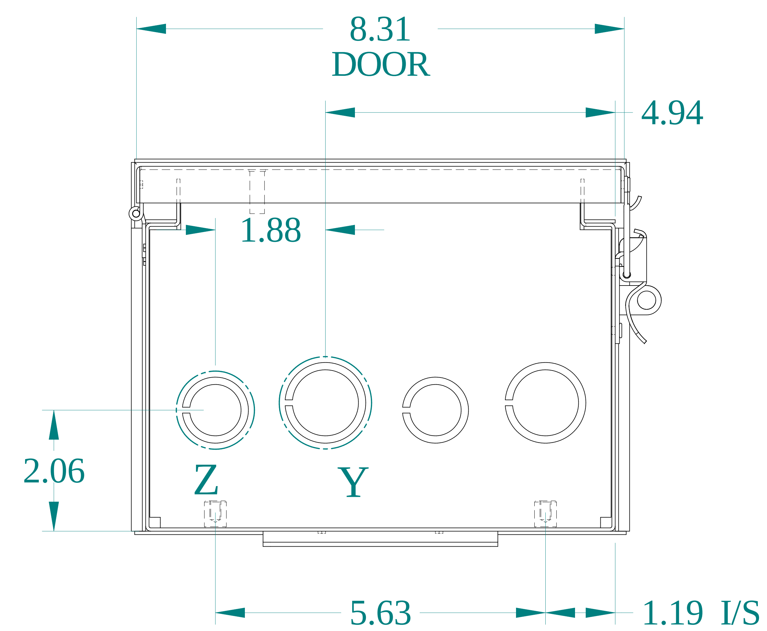
BOTTOM VIEW
