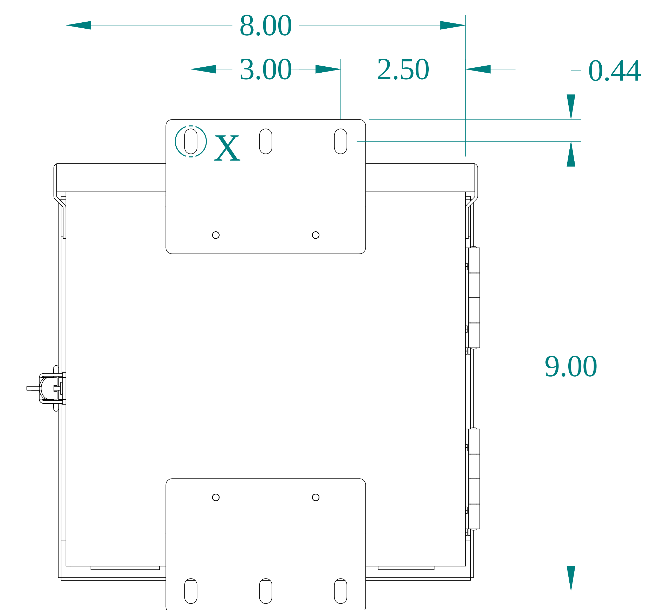
BACK VIEW
