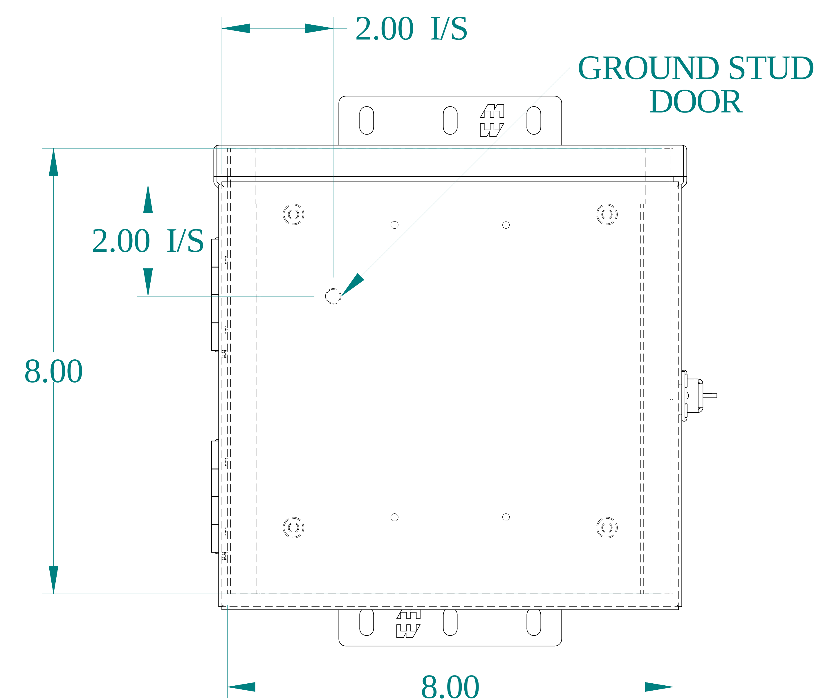
FRONT VIEW
