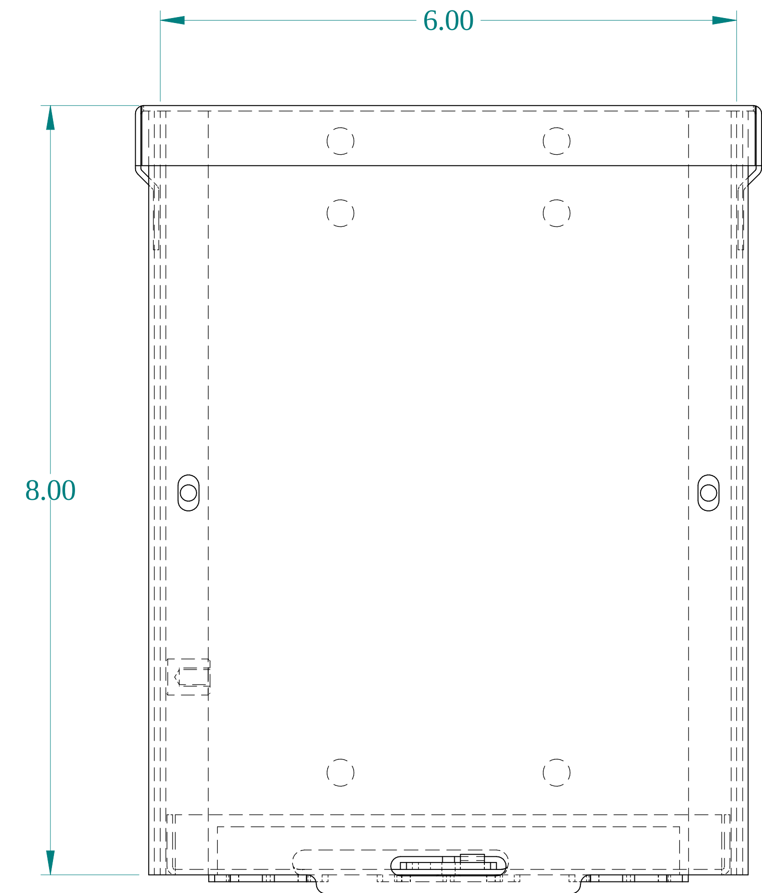
FRONT VIEW
