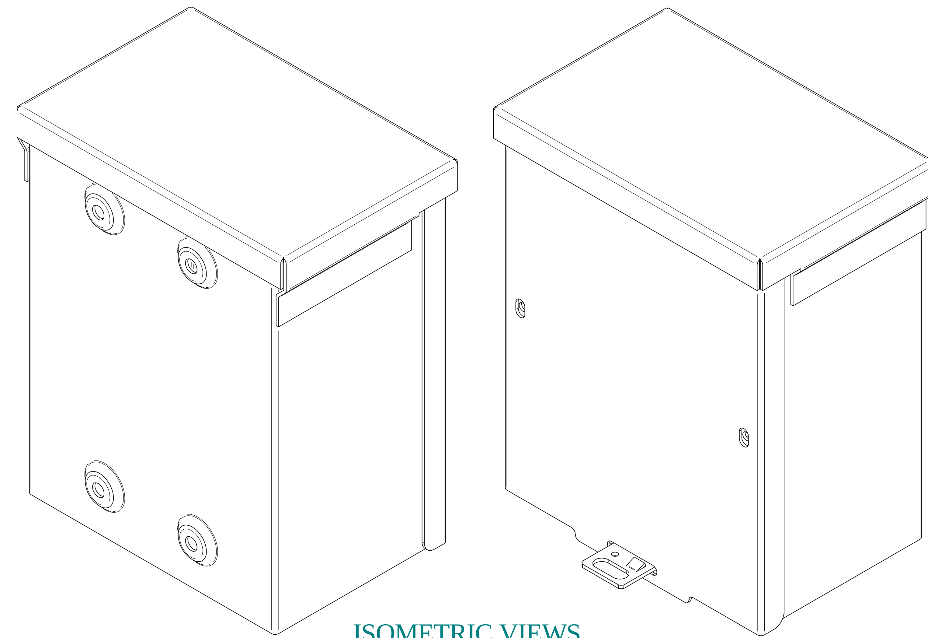
ISOMETRIC VIEWS
