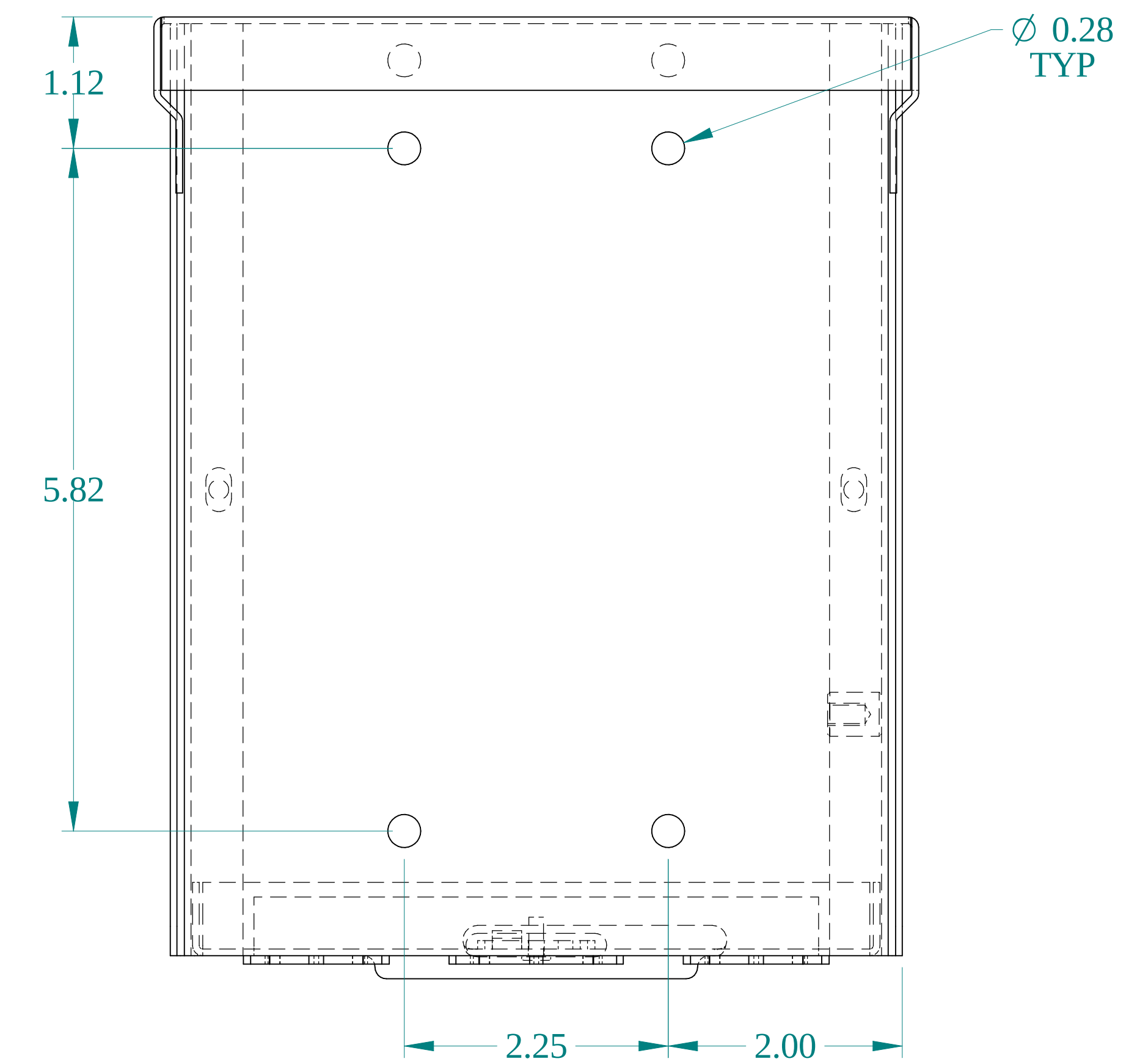
BACK VIEW
