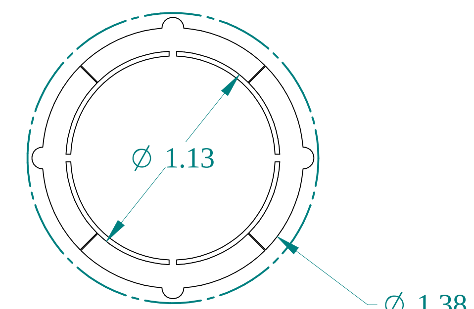
DETAIL Z
