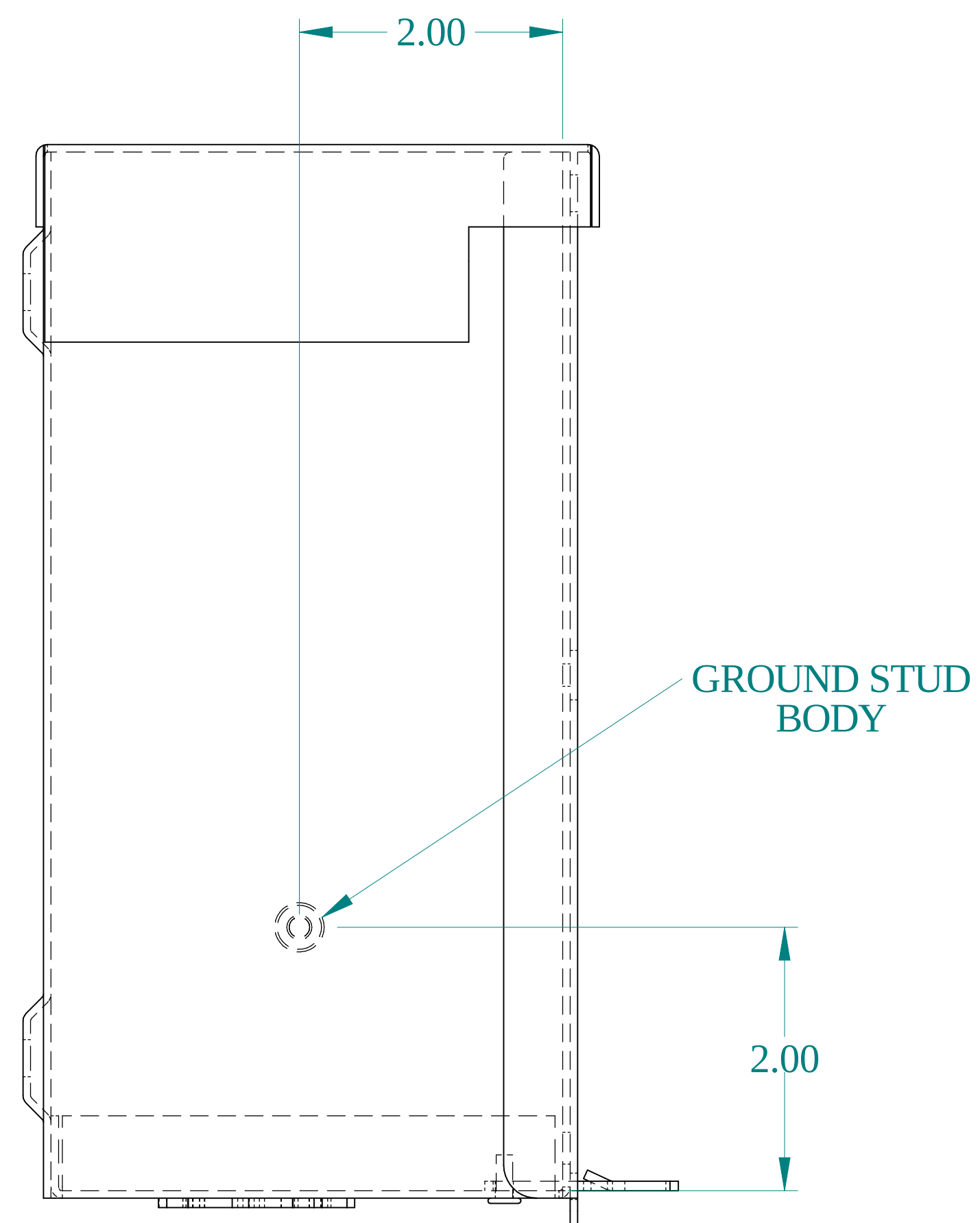
SIDE VIEW
