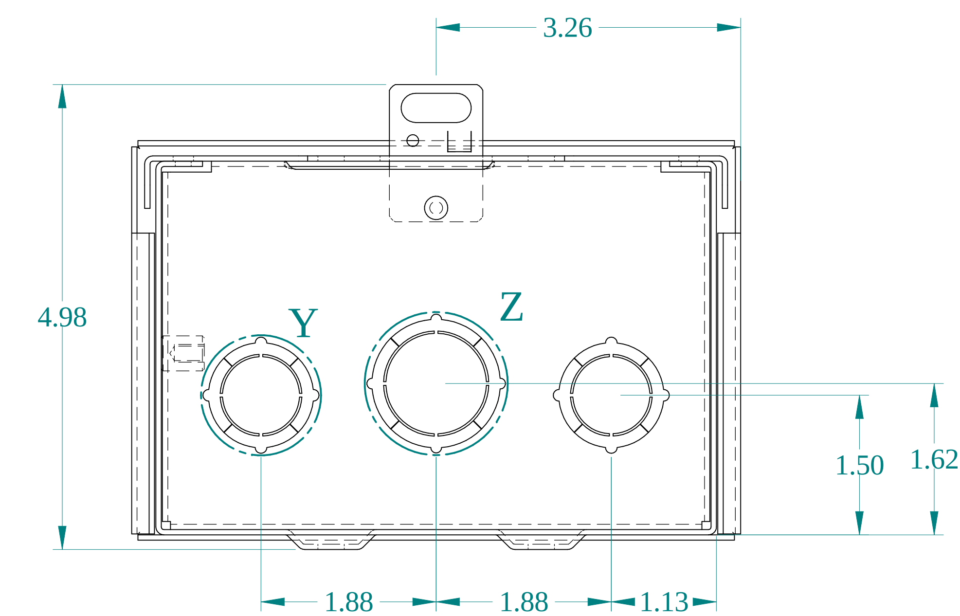
BOTTOM VIEW
