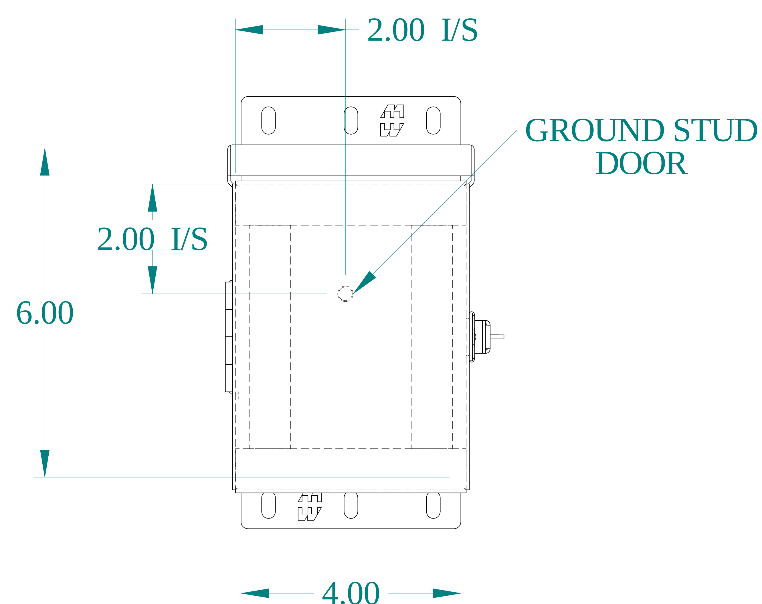
FRONT VIEW
