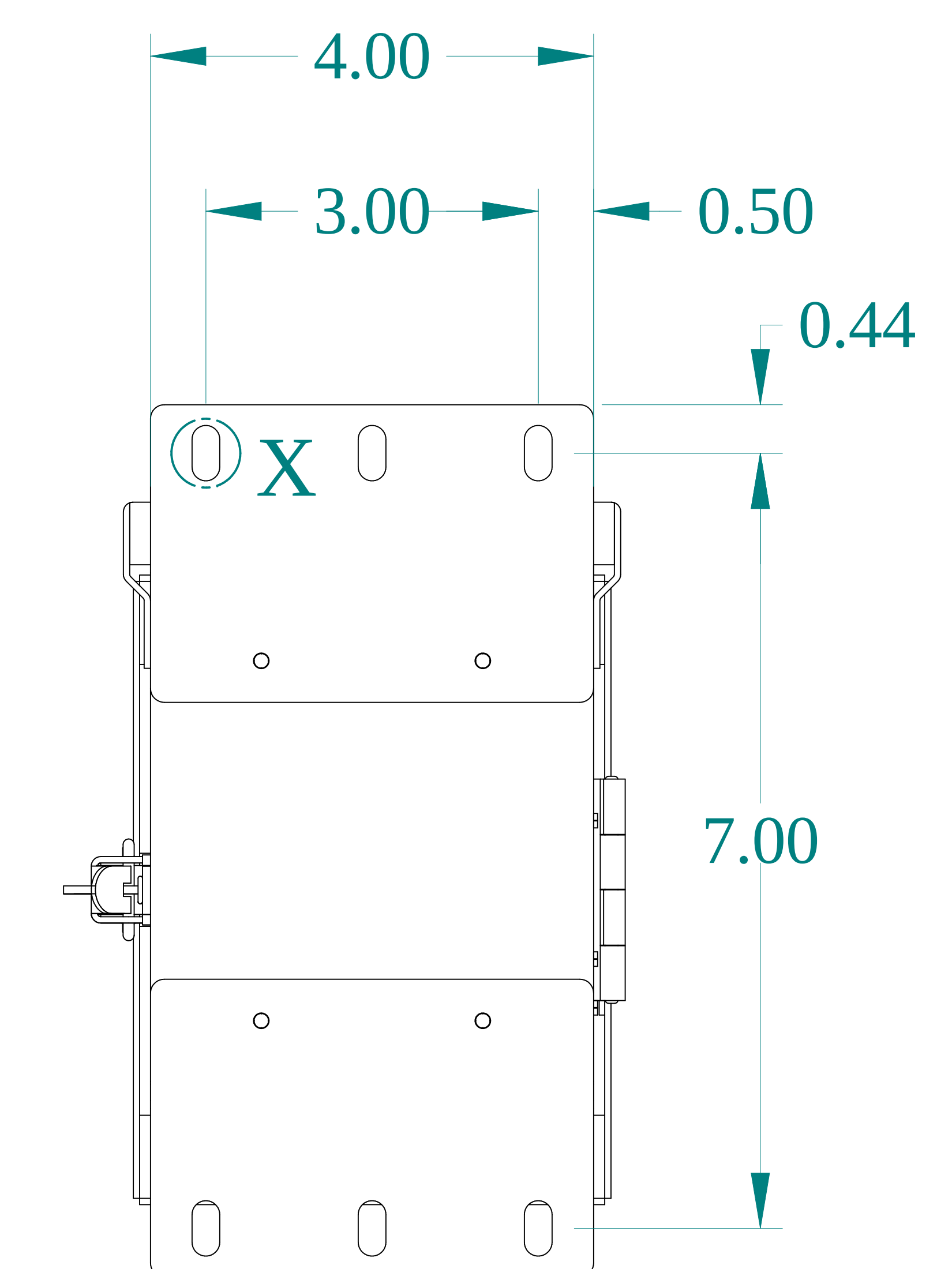
BACK VIEW
