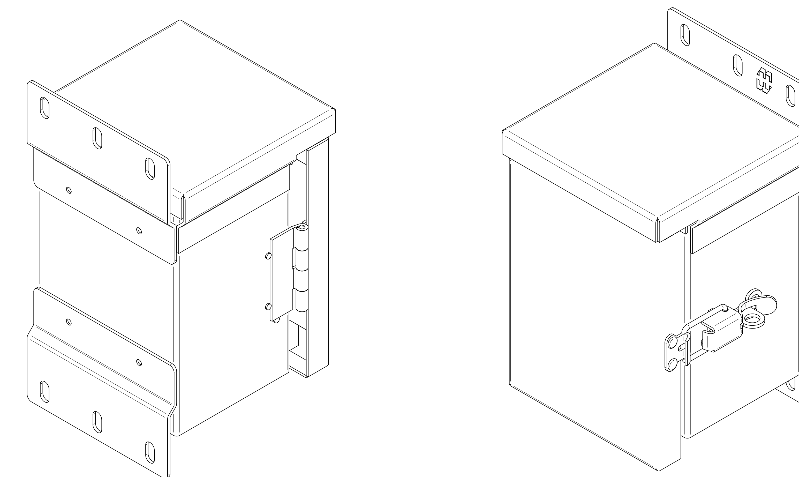
ISOMETRIC VIEWS
