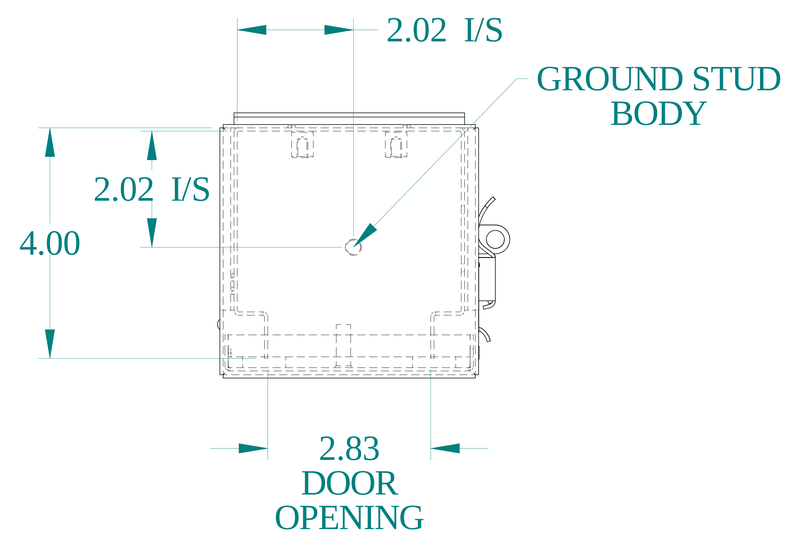
TOP VIEW
