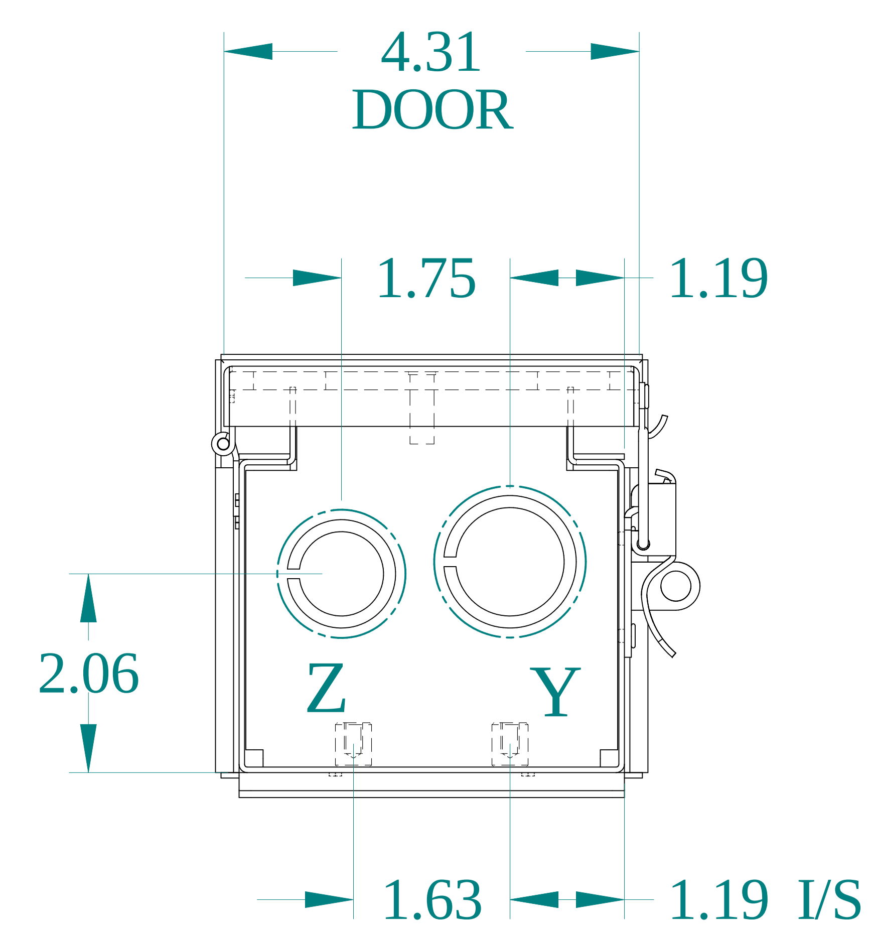
BOTTOM VIEW
