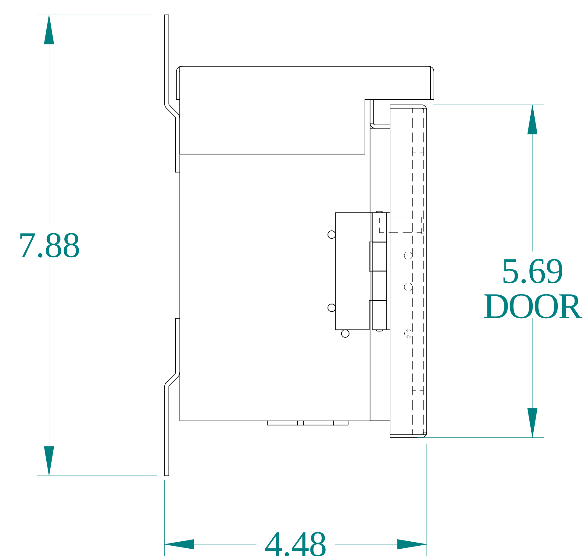
SIDE VIEW
