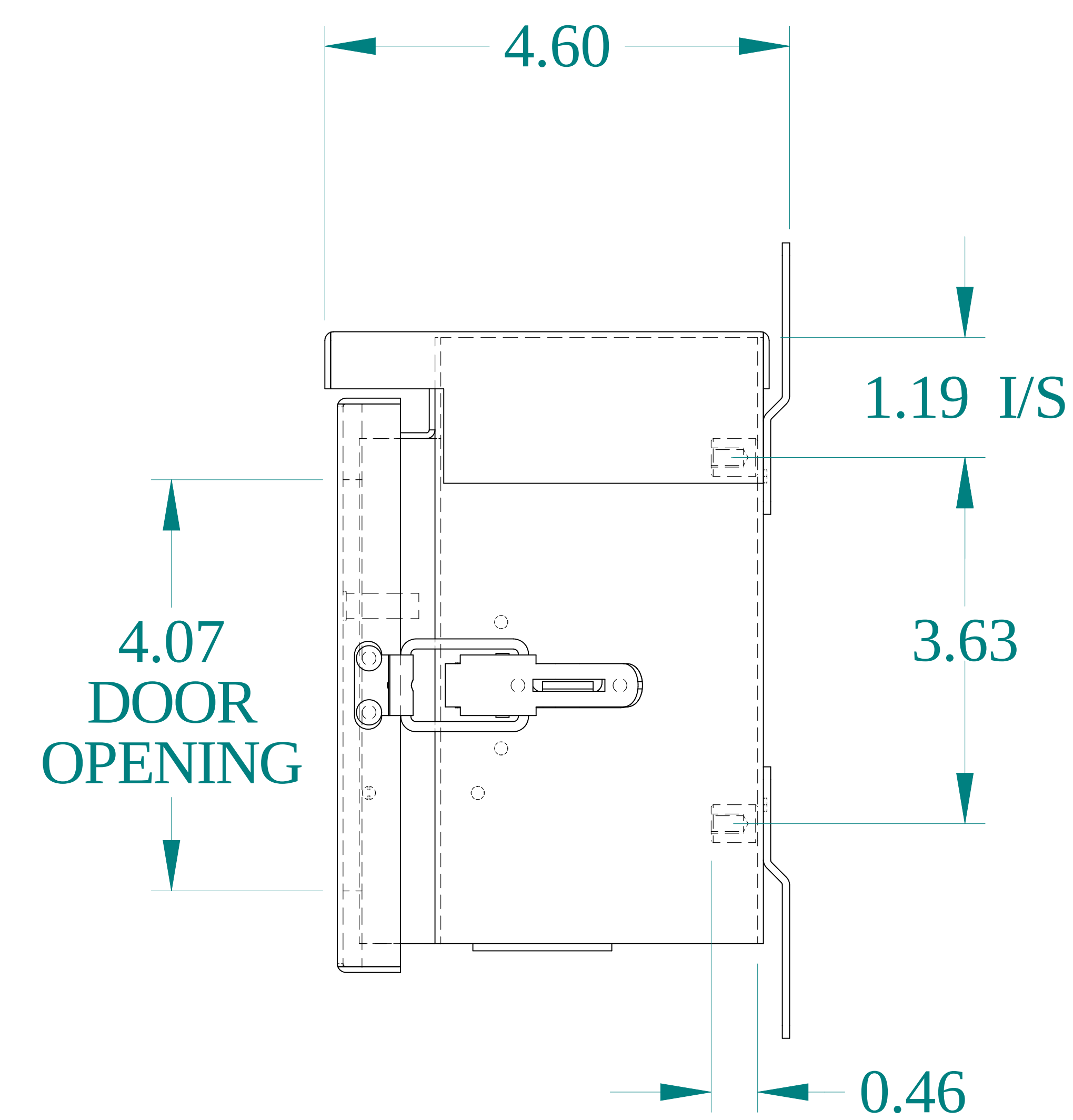
SIDE VIEW
