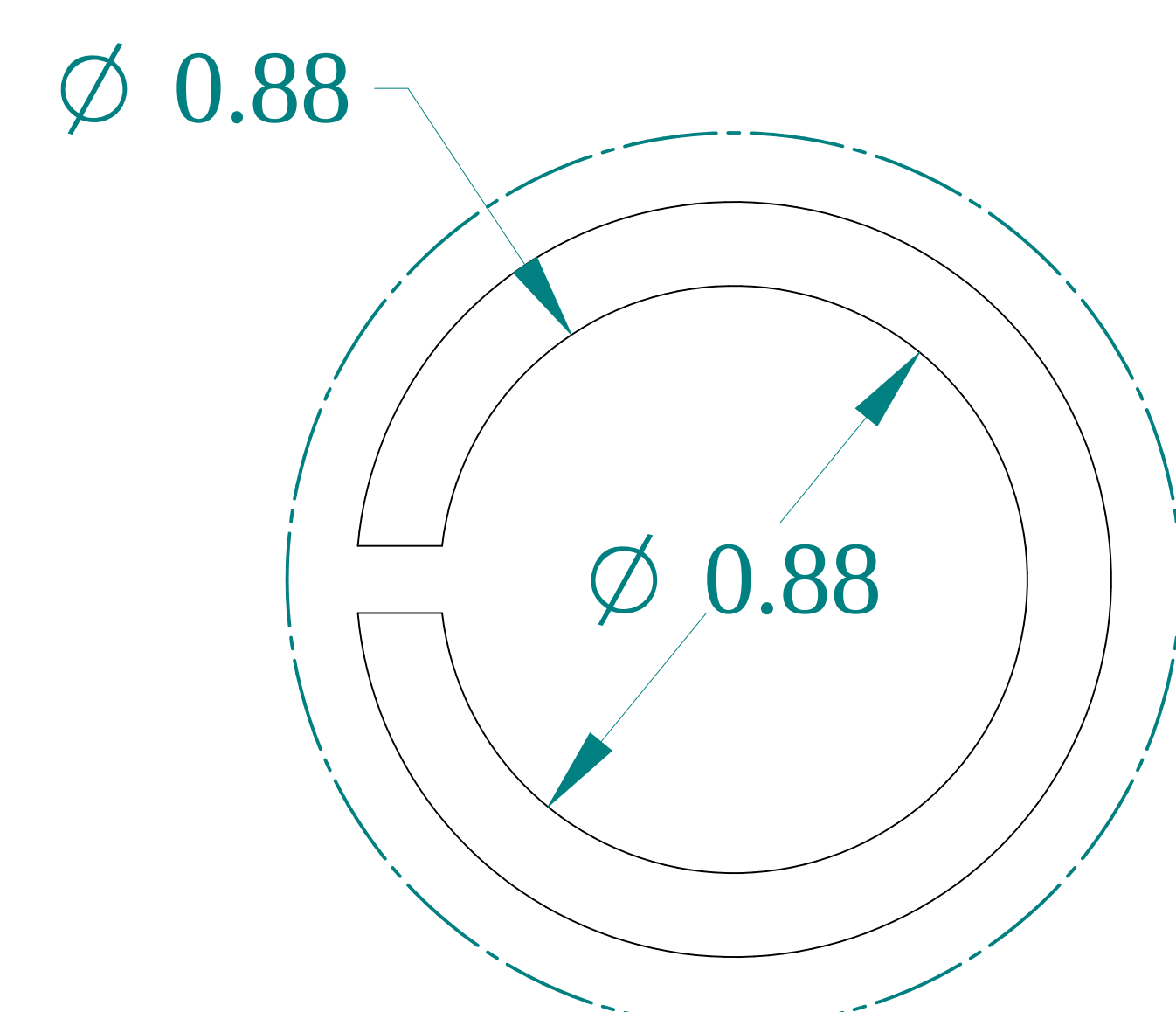
DETAIL Z
