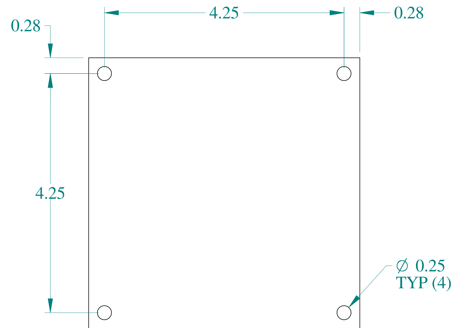
FRONT VIEW
