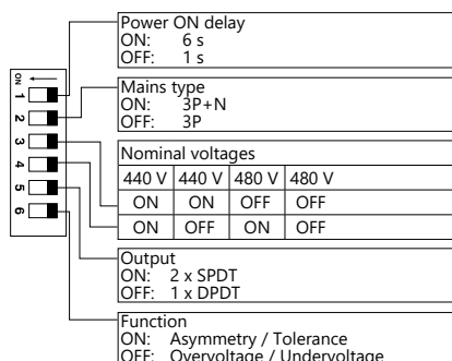
Fig. 5 DIP switch settings M49
