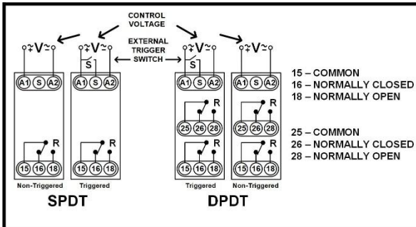
FIGURE 2: WIRING DIAGRAMS
