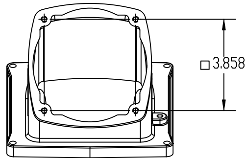
VIEW A-A 60°
