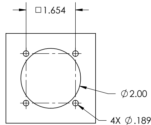
ENTRY HOLE PATTERN
