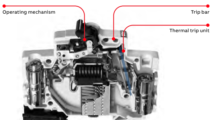
All highlighted components are energized during operation
