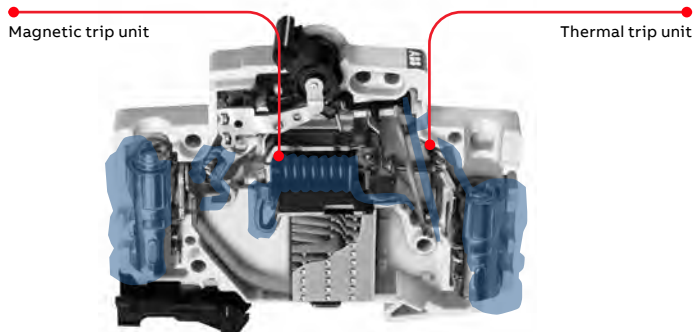
All highlighted components are energized during operation
