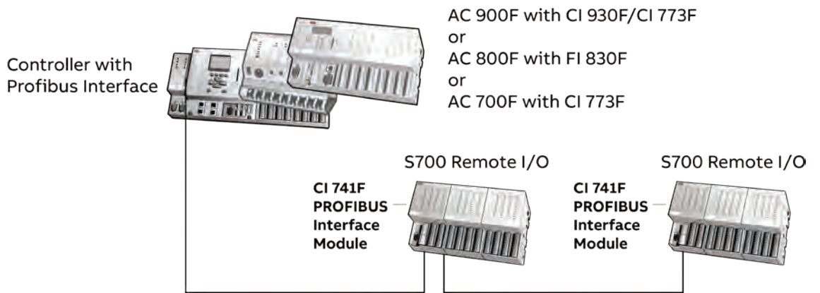
— PROFIBUS configuration with AC 900F, AC 700F, S700 remote I/O and standard PROFIBUS cable and plugs
