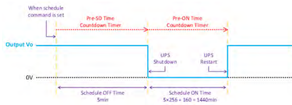
Figure 15: Timing Diagram 1.0
