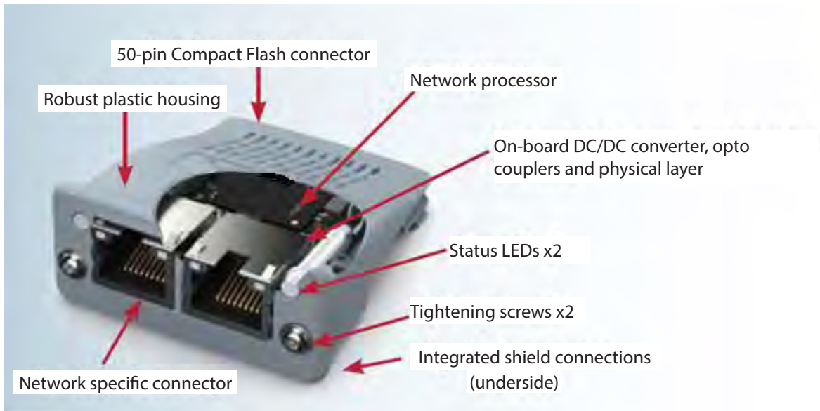
Figure 3: SDUENETIPCARD Construction
