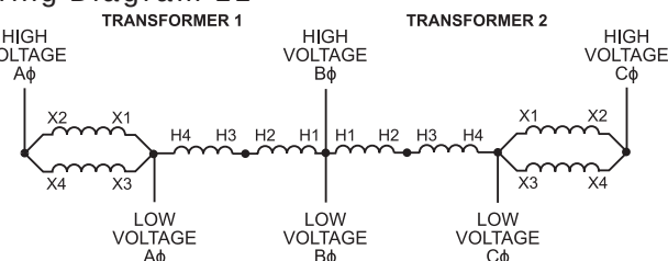
Wiring Diagram 11
