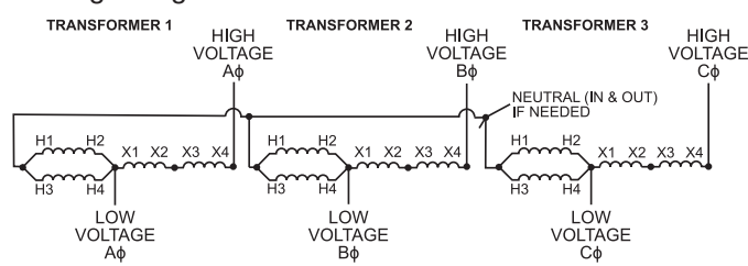
Wiring Diagram 8
