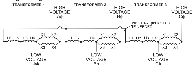
Wiring Diagram 7
