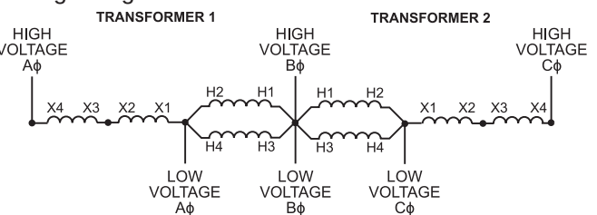
Wiring Diagram 12
