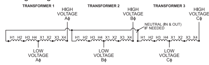
Wiring Diagram 8
