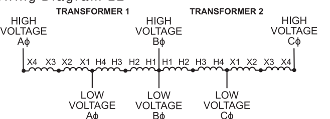
Wiring Diagram 12
