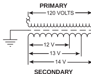
S120A Wiring Diagram & Connections
