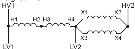
Wiring Diagram 3
