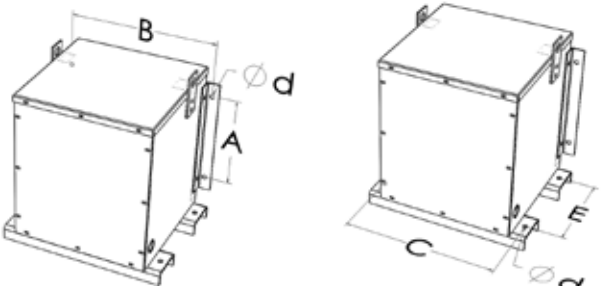
Diagram: Wall Mounting
