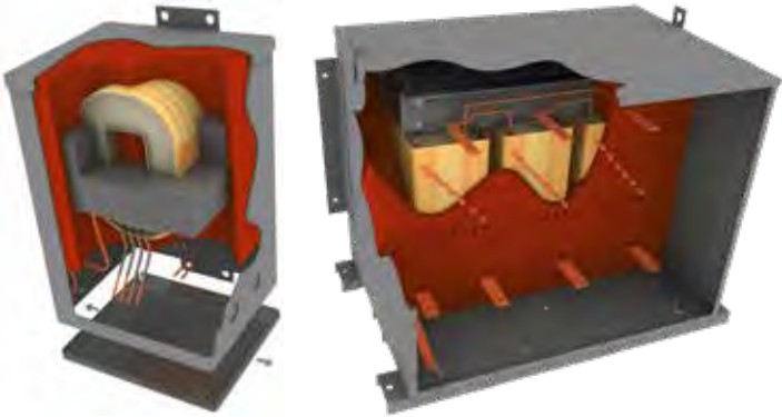
Construction Type 1 Single Phase units Wiring Compartment is located at underside Construction Type 2 Three Phase units Wiring Compartment is located at front
