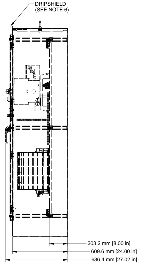
SIDE VIEW SCALE 1/20
