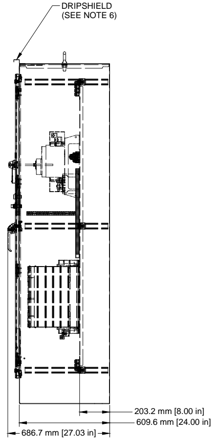
SIDE VIEW SCALE 1 / 20
