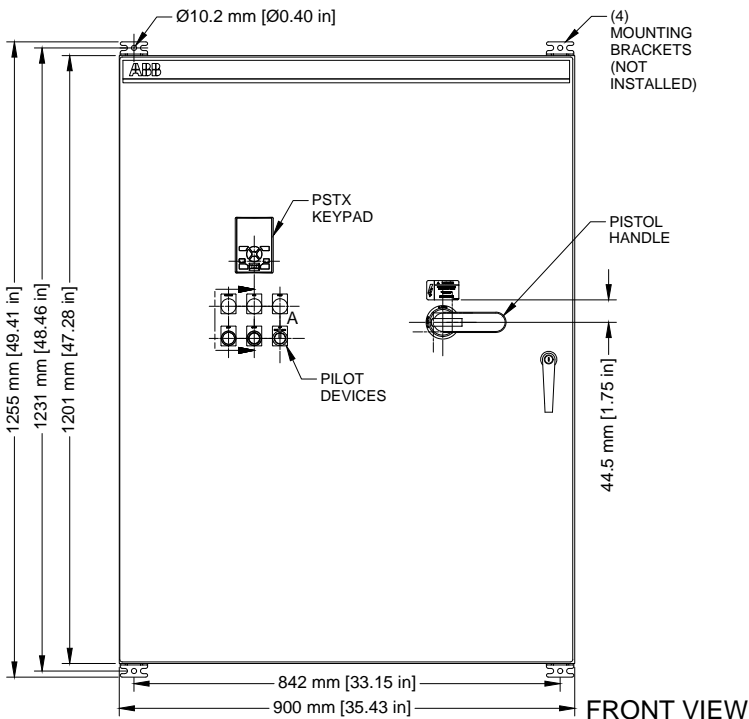
FRONT VIEW SCALE 1 / 12
