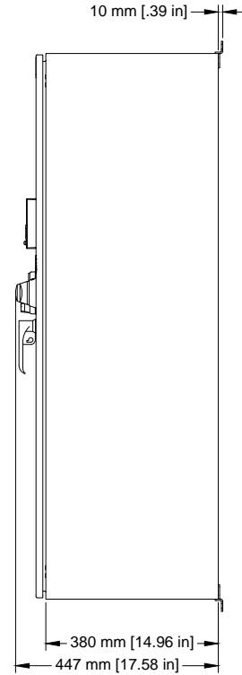
SIDE VIEW SCALE 1 / 12
