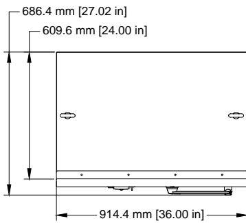
TOP VIEW SCALE 1/20
