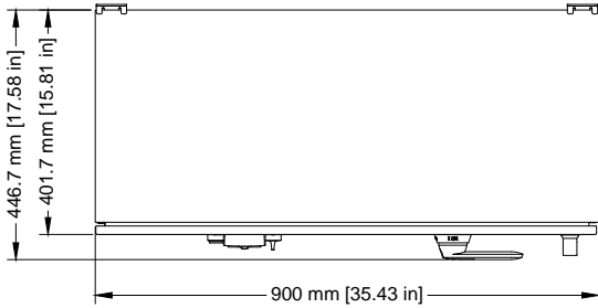
TOP VIEW SCALE 1 / 12
