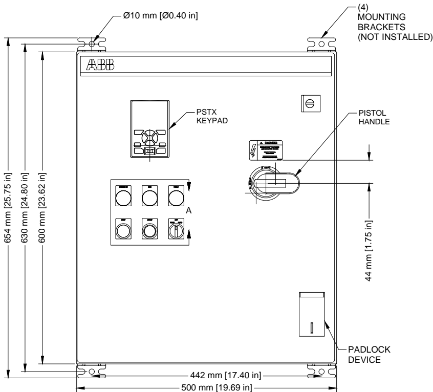
FRONT VIEW SCALE 1 / 6
