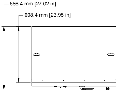
TOP VIEW SCALE 1 / 20
