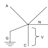
3 PHASE WYE 4 WIRE + GROUND
