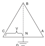
HI-LEG GROUNDED DELTA
