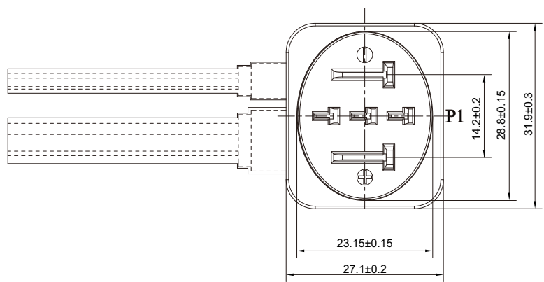
EBSP Battery Discharging Plug
