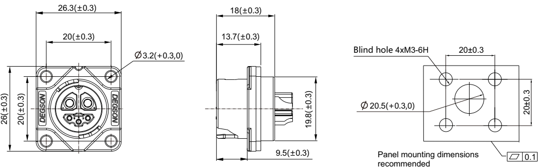
EBBM Socket
