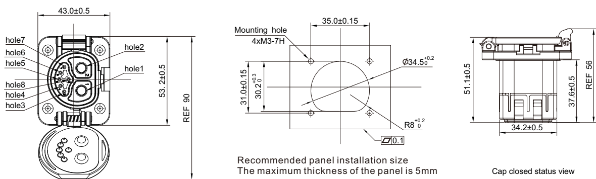
EBBH 80A power socket with cover flap
