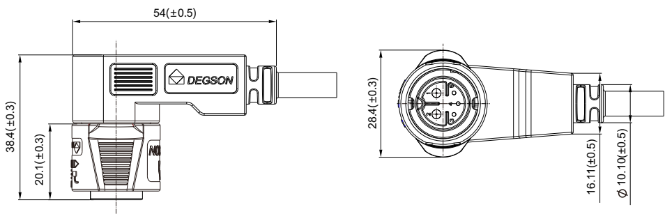
EBBM Right Angle Plug
