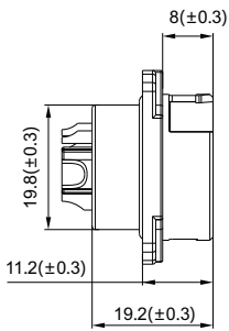
EBBL Socket
