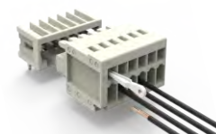
Cage springs
