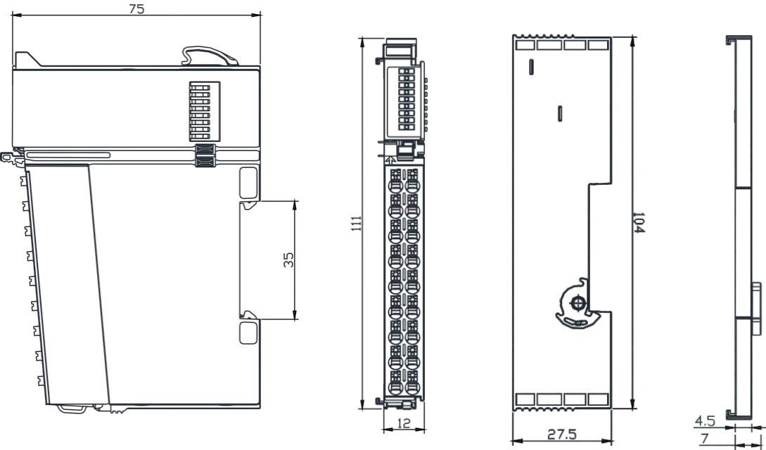
DF50 series I/O module & Terminal cover dimension
