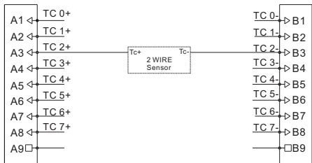
Wiring Diagram
