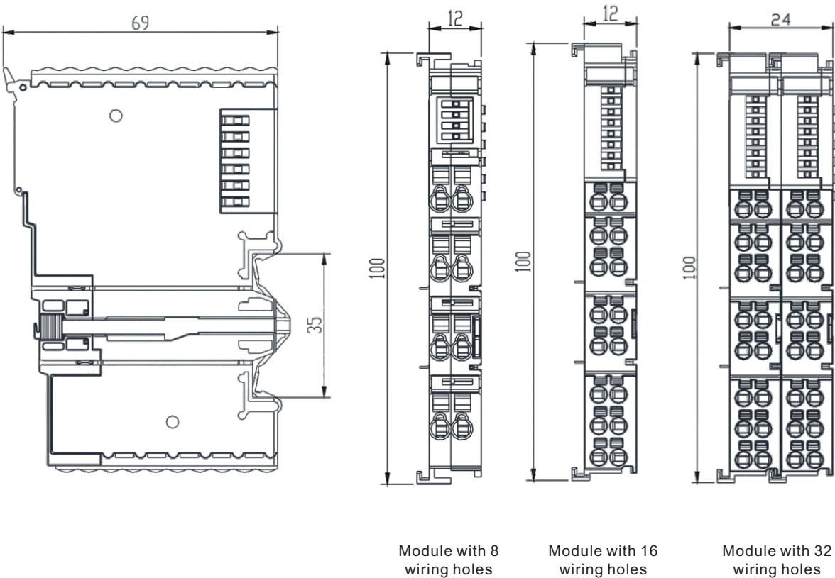
DF20 series I/O module dimension
