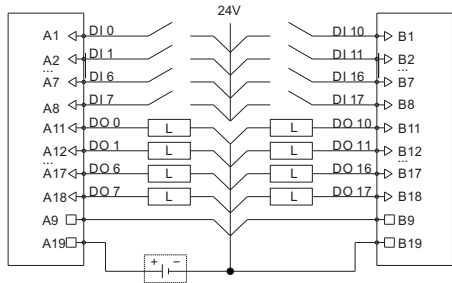
Wiring Diagram
