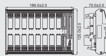
DM108-RM-32-PN-2-4M-100Z(H)
