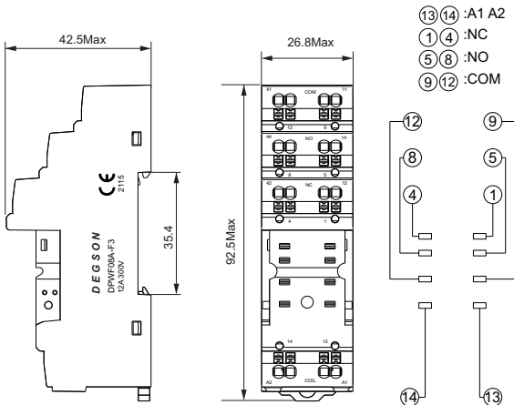
DPWF08A-F3
