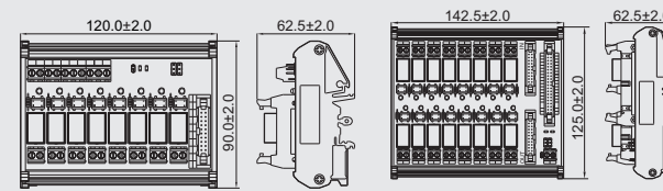
DM72-RMS-08-PN-1-4M-00Z(H)
