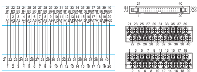
DM50-IDC-40-40-4G-00Z(H)
