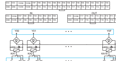
DM108-RM-16-PN-2-4M-100Z(H)
