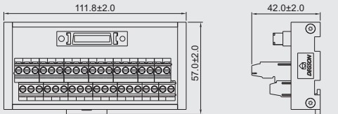
DM50-IDC-36-36-4Y-00Z(H)
