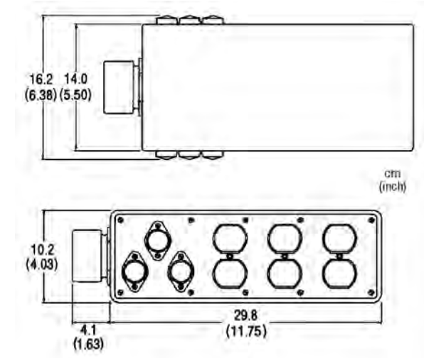
Multiple Outlet Box, Series 3100
