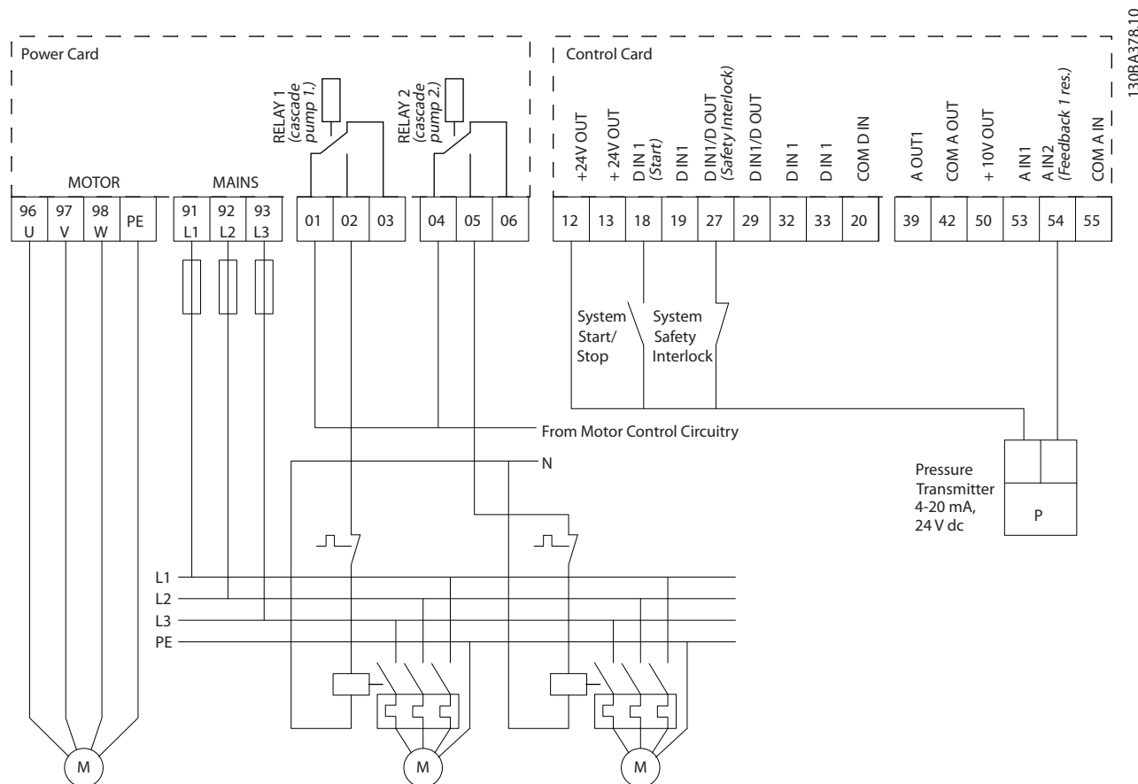
Illustration 12.6 Cascade Controller Wiring Diagram
