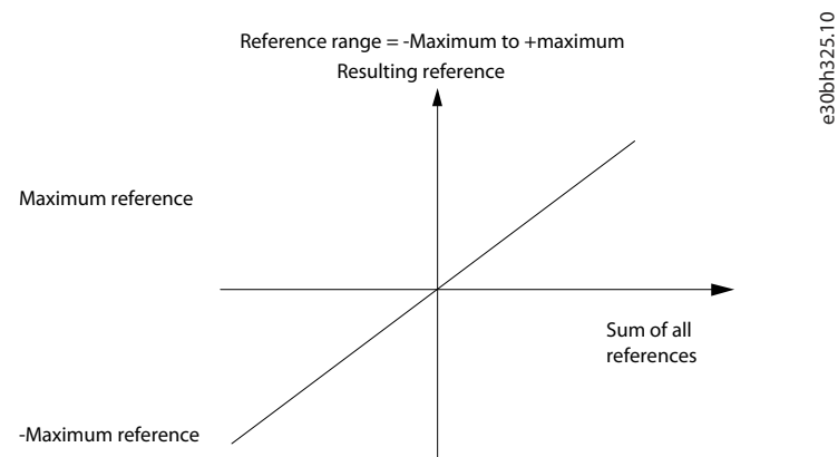
Illustration 88: Sum of All References When Reference Range is Set to 1
