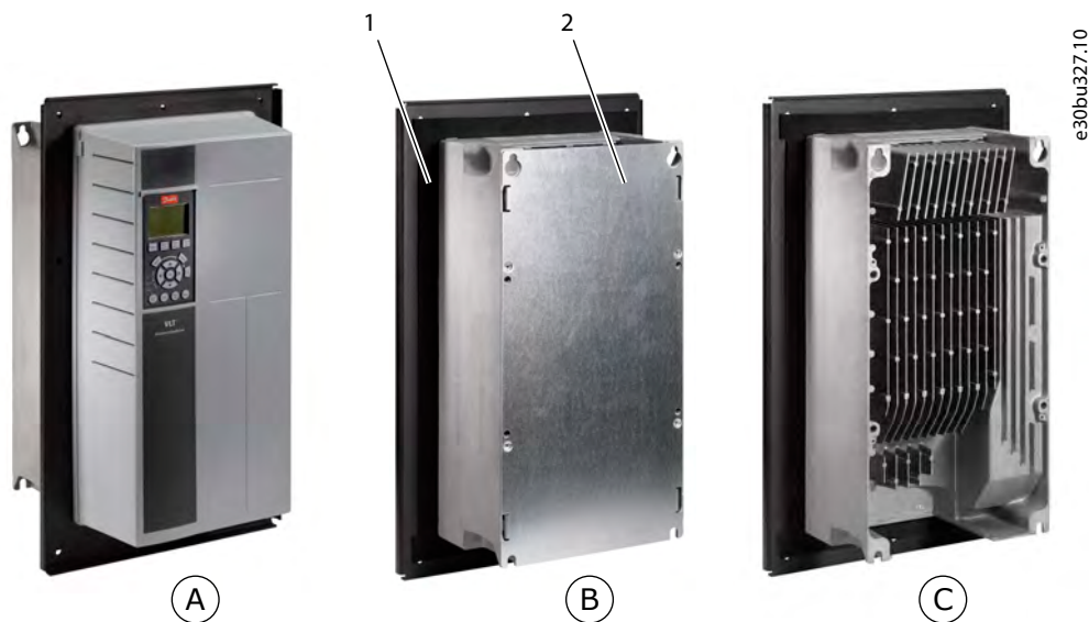
Illustration 42: Panel Through Mounting Kit on VLT® AutomationDrive FC 302
