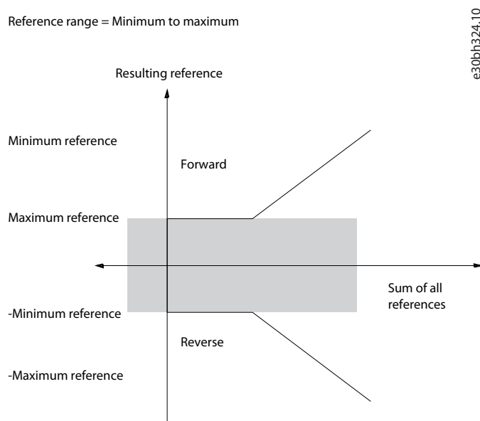
Illustration 87: Sum of All References When Reference Range is Set to 0
