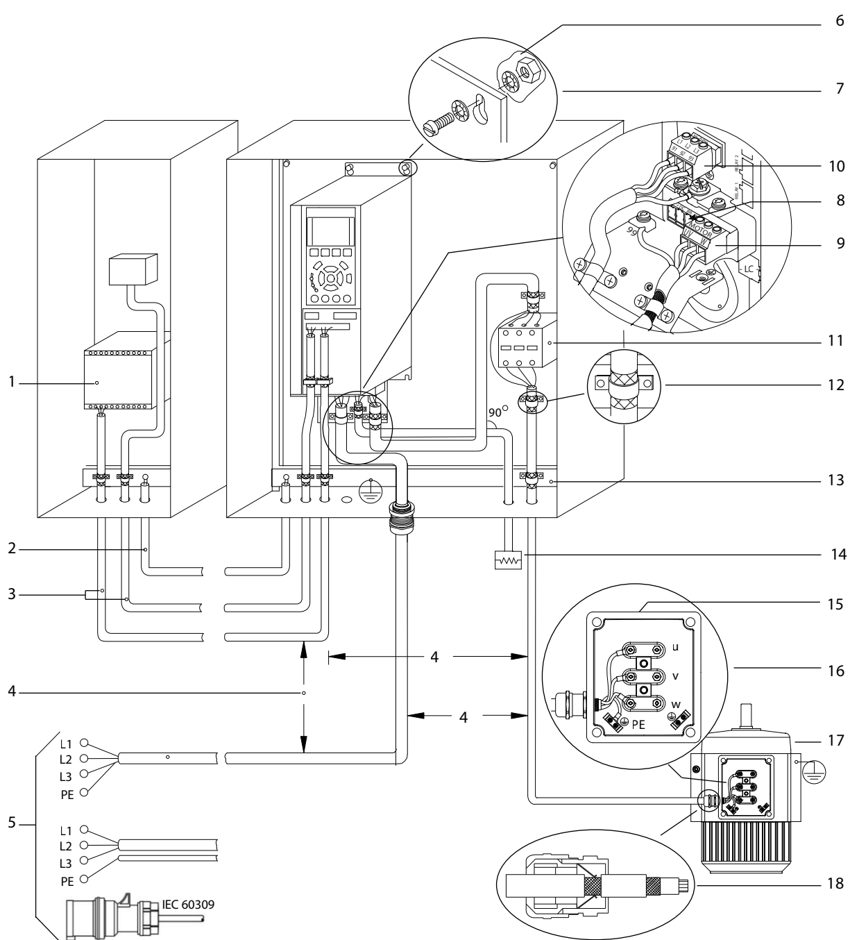
Illustration 60: EMC-compliant Electrical Connection
