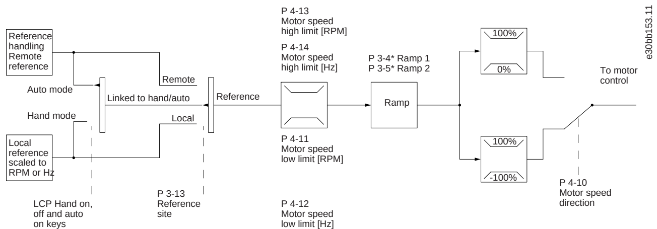
Illustration 91: Open-loop Structure
