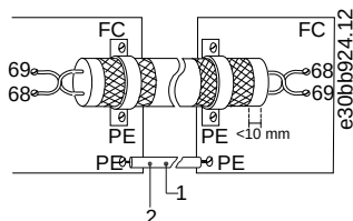
Illustration 67: Twisted-pair Cables without Terminal 61
