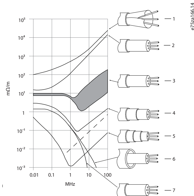
Illustration 63: Transfer Impedance ( Z_T )
