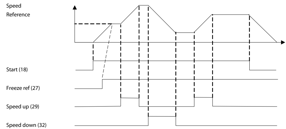
Illustration 93: Speed Up/Down
