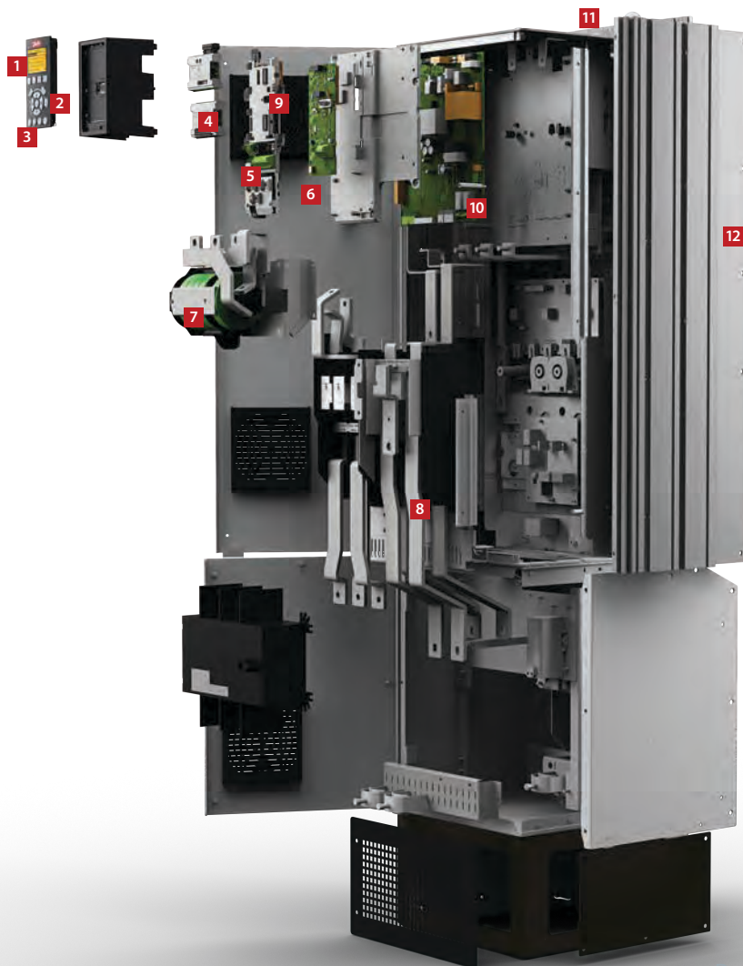
Enclosure size D, IP54
