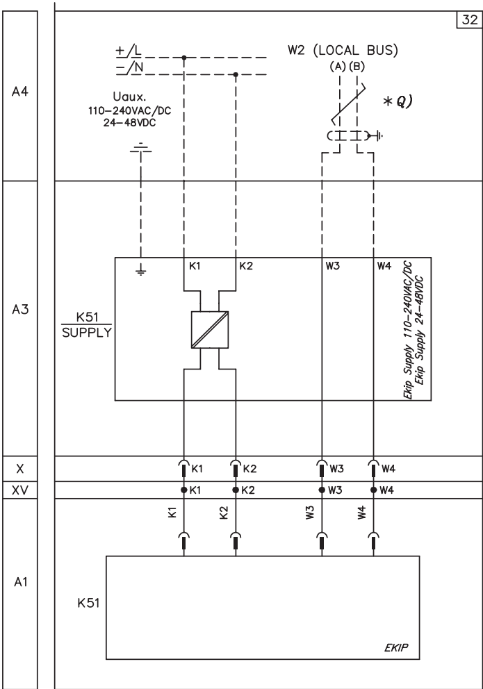
32) Auxiliary supply through module 110-240V AC/DC or 24-48V DC and local bus - Ekip Supply
