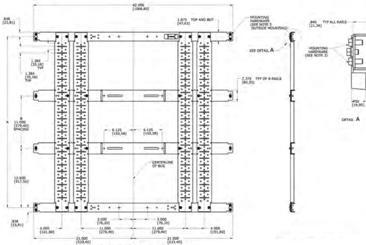
45 IN. WIDE ENCLOSURE CENTER FRAME 24X LENGTH SHOWN
