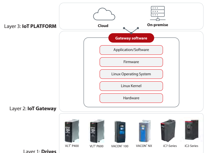
Figure 1: Layers of the DrivePro® Remote Monitoring solution
