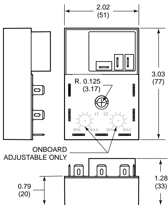
All Dimensions in Inches (Millimeters)
