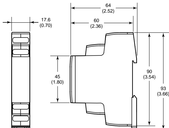
All Dimensions in Inches (Millimeters)
