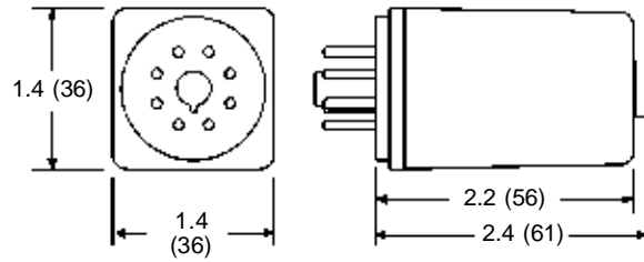
All Dimensions in Inches (Millimeters)
