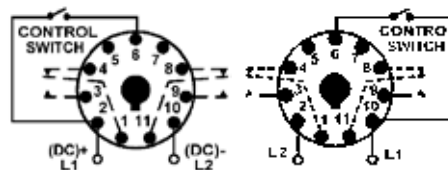
Standard 11 pin modified with a 2-6 control switch (Suffix T2)
