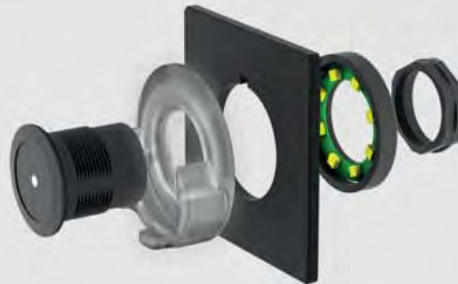
Holder for RFID reader with LED status indication
