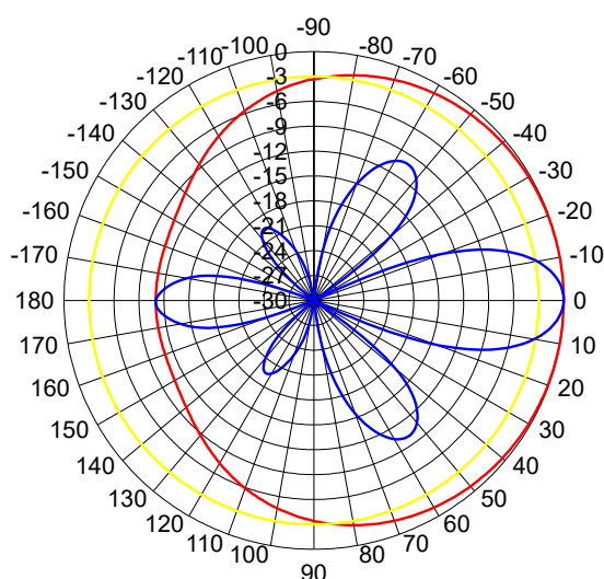
RADIATION PATTERN
