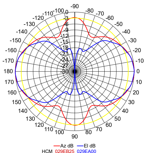
CS-power splitter required in circular mode RADIATION PATTERN, CIRCULAR
