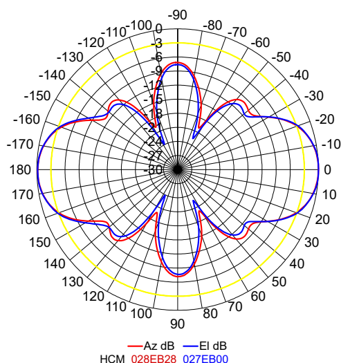
RADIATION PATTERN, SLANTED
