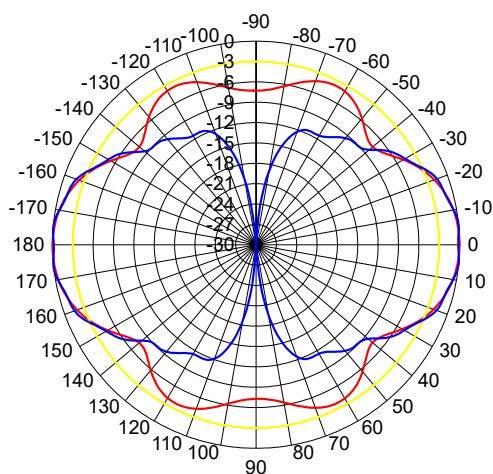
RADIATION PATTERN, CIRCULAR
