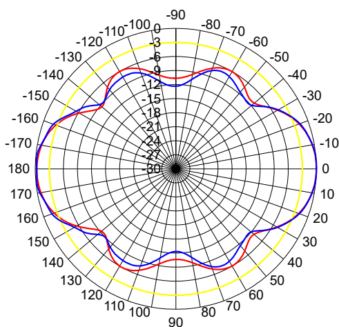
RADIATION PATTERN, SLANTED
